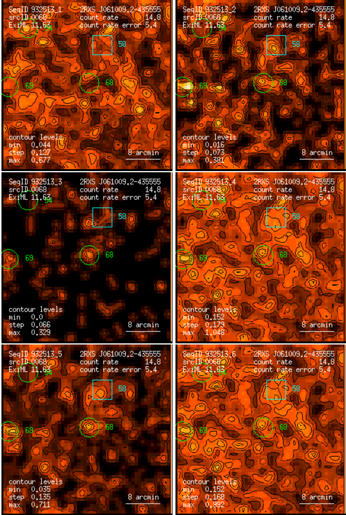
Figure 68: RASS 932513: detection 0068: band rate images, Gaussian filter: (1) PSPC channels 11 – 41, (2) 52 – 90, (3) 91 – 201, (4) 11 – 235, (5) 52 – 201, (6) 11 – 201. Broad band rates in counts/ks. Band rate contour levels in counts/ks/arcmin 2 .
