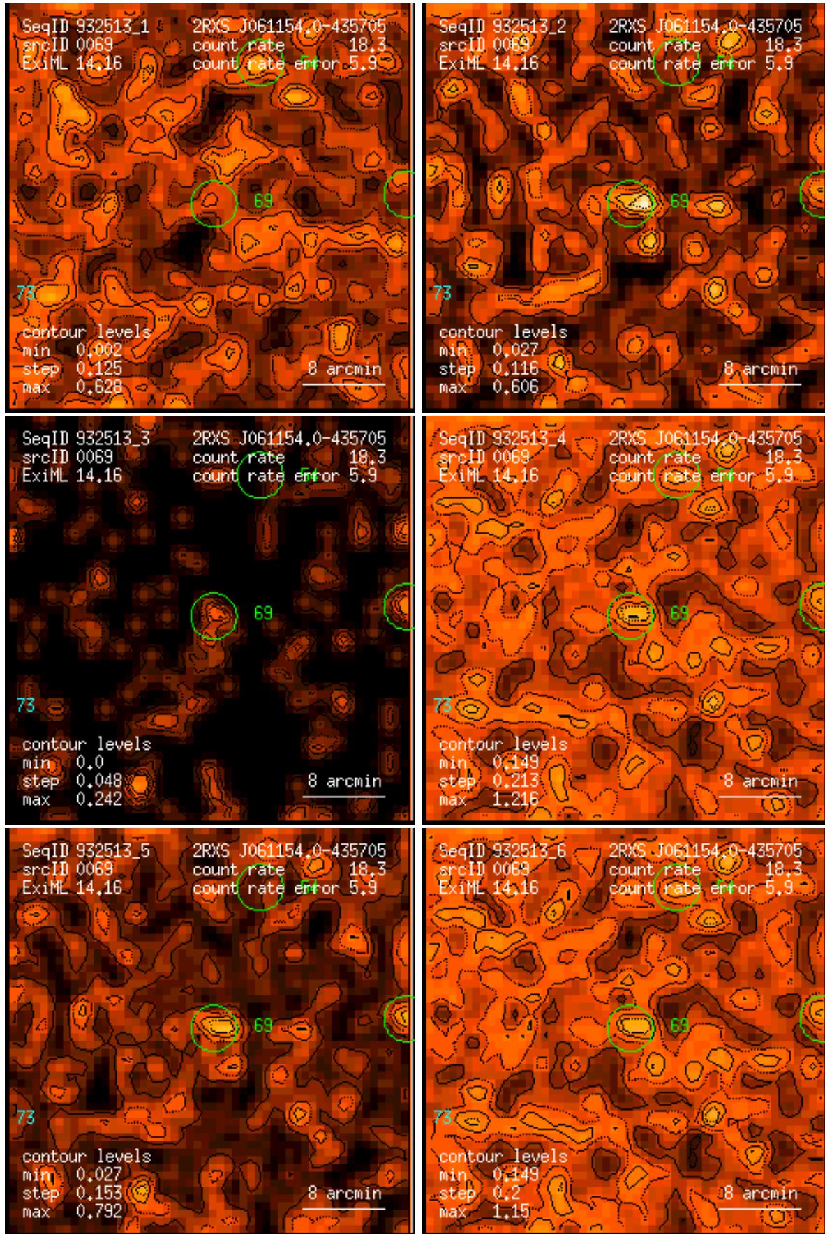
Figure 69: RASS 932513: detection 0069: band rate images, Gaussian filter: (1) PSPC channels 11 – 41, (2) 52 – 90, (3) 91 – 201, (4) 11 – 235, (5) 52 – 201, (6) 11 – 201. Broad band rates in counts/ks. Band rate contour levels in counts/ks/arcmin 2 .
