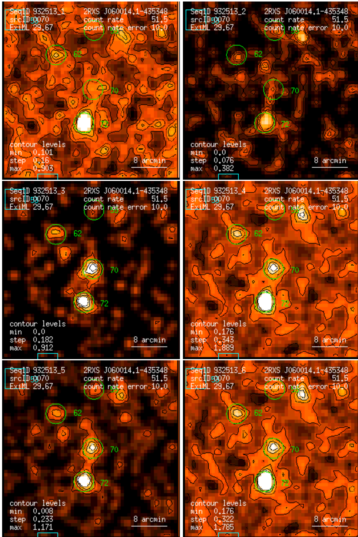
Figure 70: RASS 932513: detection 0070: band rate images, Gaussian filter: (1) PSPC channels 11 – 41, (2) 52 – 90, (3) 91 – 201, (4) 11 – 235, (5) 52 – 201, (6) 11 – 201. Broad band rates in counts/ks. Band rate contour levels in counts/ks/arcmin 2 .
