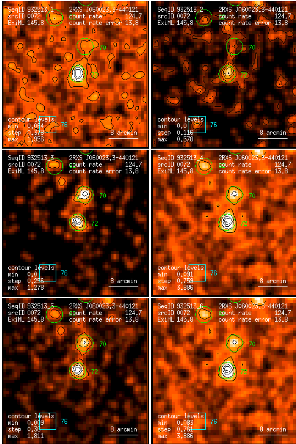
Figure 72: RASS 932513: detection 0072: band rate images, Gaussian filter: (1) PSPC channels 11 – 41, (2) 52 – 90, (3) 91 – 201, (4) 11 – 235, (5) 52 – 201, (6) 11 – 201. Broad band rates in counts/ks. Band rate contour levels in counts/ks/arcmin 2 .
