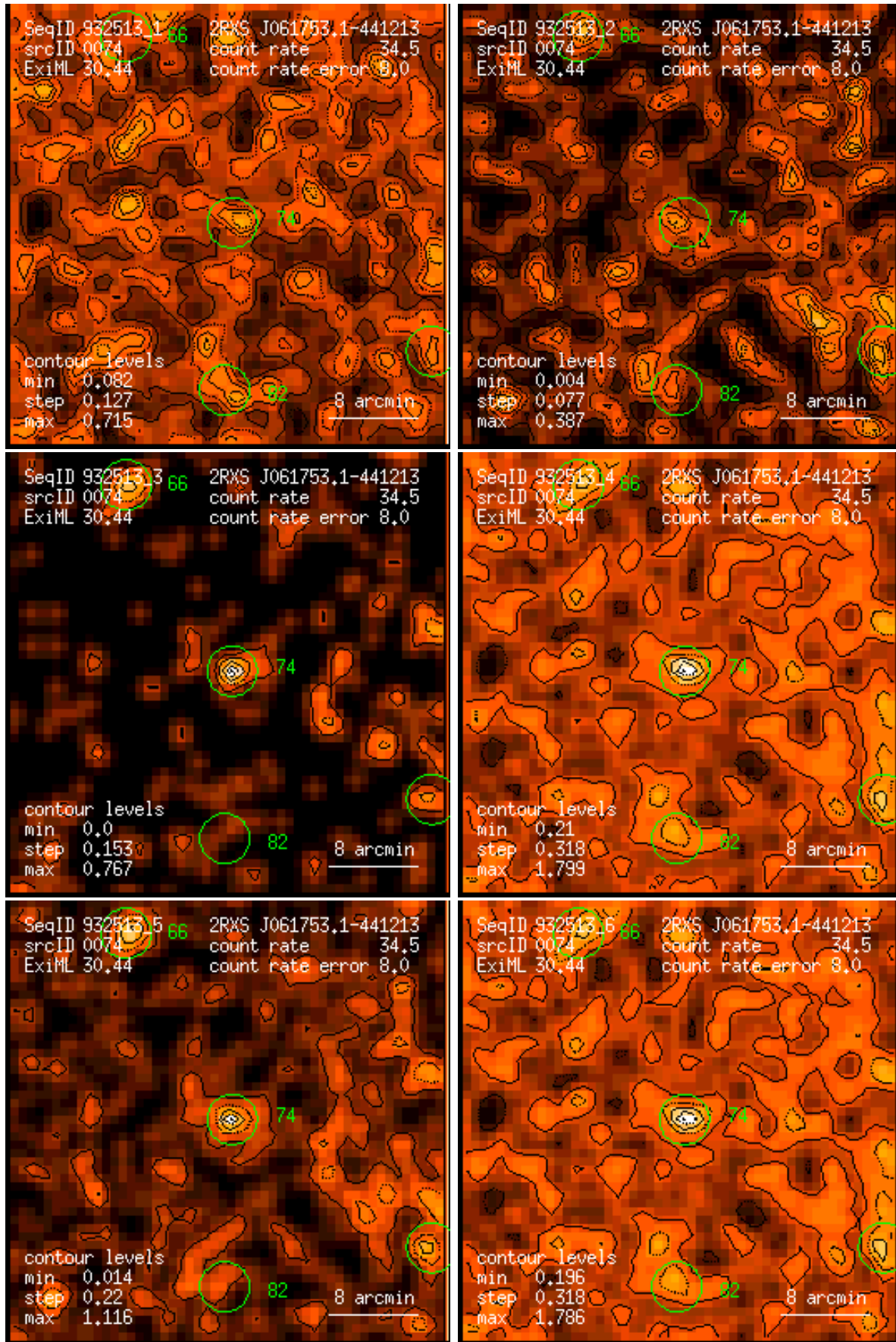
Figure 74: RASS 932513: detection 0074: band rate images, Gaussian filter: (1) PSPC channels 11 – 41, (2) 52 – 90, (3) 91 – 201, (4) 11 – 235, (5) 52 – 201, (6) 11 – 201. Broad band rates in counts/ks. Band rate contour levels in counts/ks/arcmin 2 .
