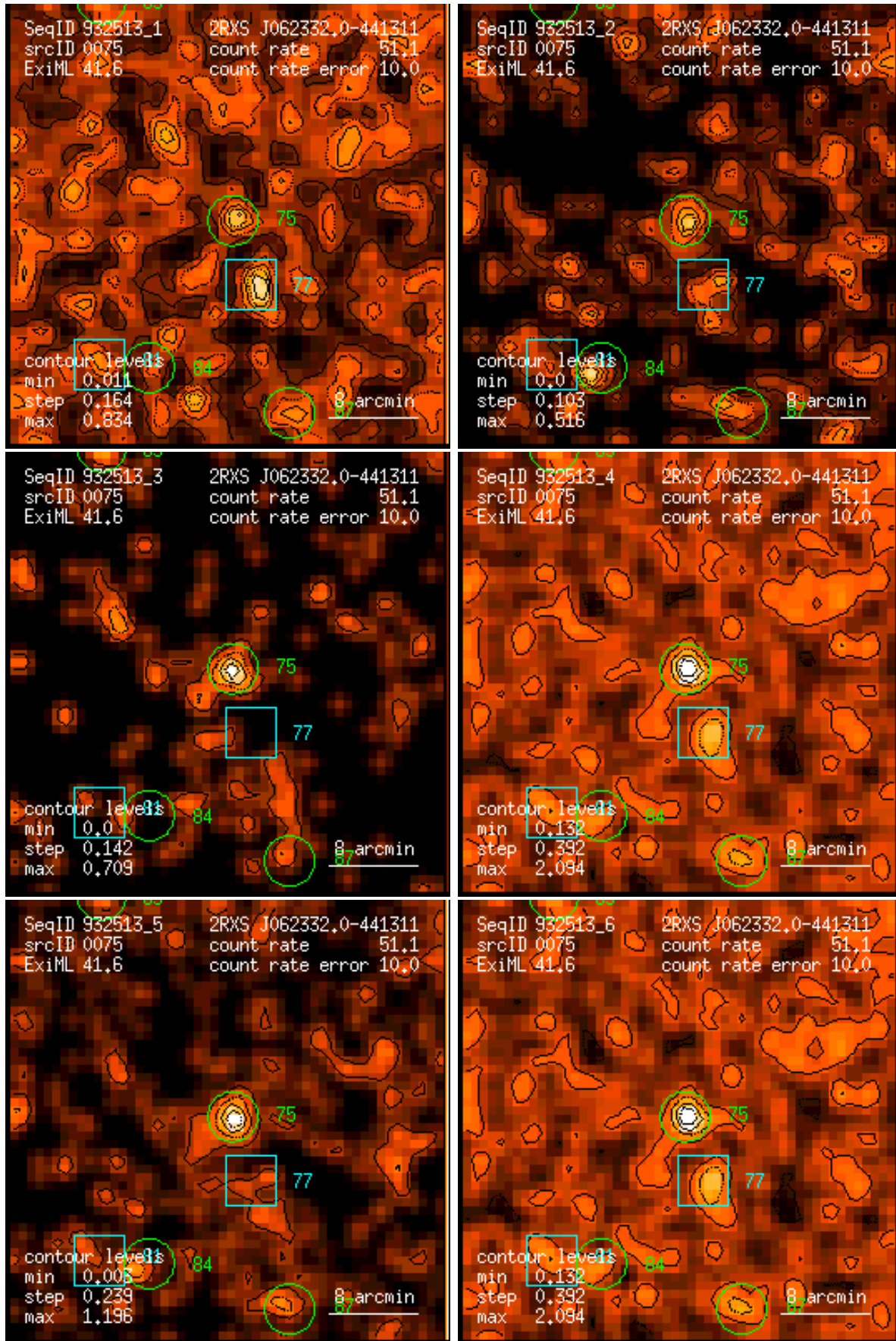
Figure 75: RASS 932513: detection 0075: band rate images, Gaussian filter: (1) PSPC channels 11 – 41, (2) 52 – 90, (3) 91 – 201, (4) 11 – 235, (5) 52 – 201, (6) 11 – 201. Broad band rates in counts/ks. Band rate contour levels in counts/ks/arcmin 2 .
