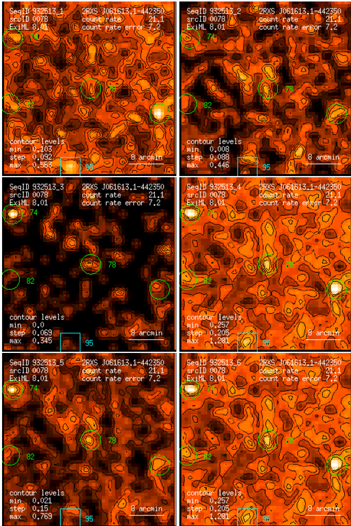
Figure 78: RASS 932513: detection 0078: band rate images, Gaussian filter: (1) PSPC channels 11 – 41, (2) 52 – 90, (3) 91 – 201, (4) 11 – 235, (5) 52 – 201, (6) 11 – 201. Broad band rates in counts/ks. Band rate contour levels in counts/ks/arcmin 2 .
