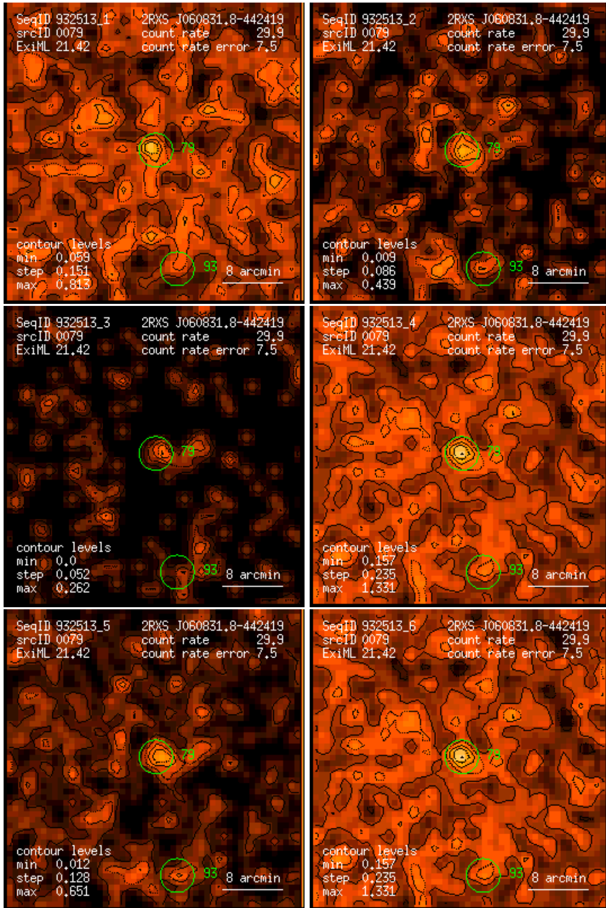
Figure 79: RASS 932513: detection 0079: band rate images, Gaussian filter: (1) PSPC channels 11 – 41, (2) 52 – 90, (3) 91 – 201, (4) 11 – 235, (5) 52 – 201, (6) 11 – 201. Broad band rates in counts/ks. Band rate contour levels in counts/ks/arcmin 2 .
