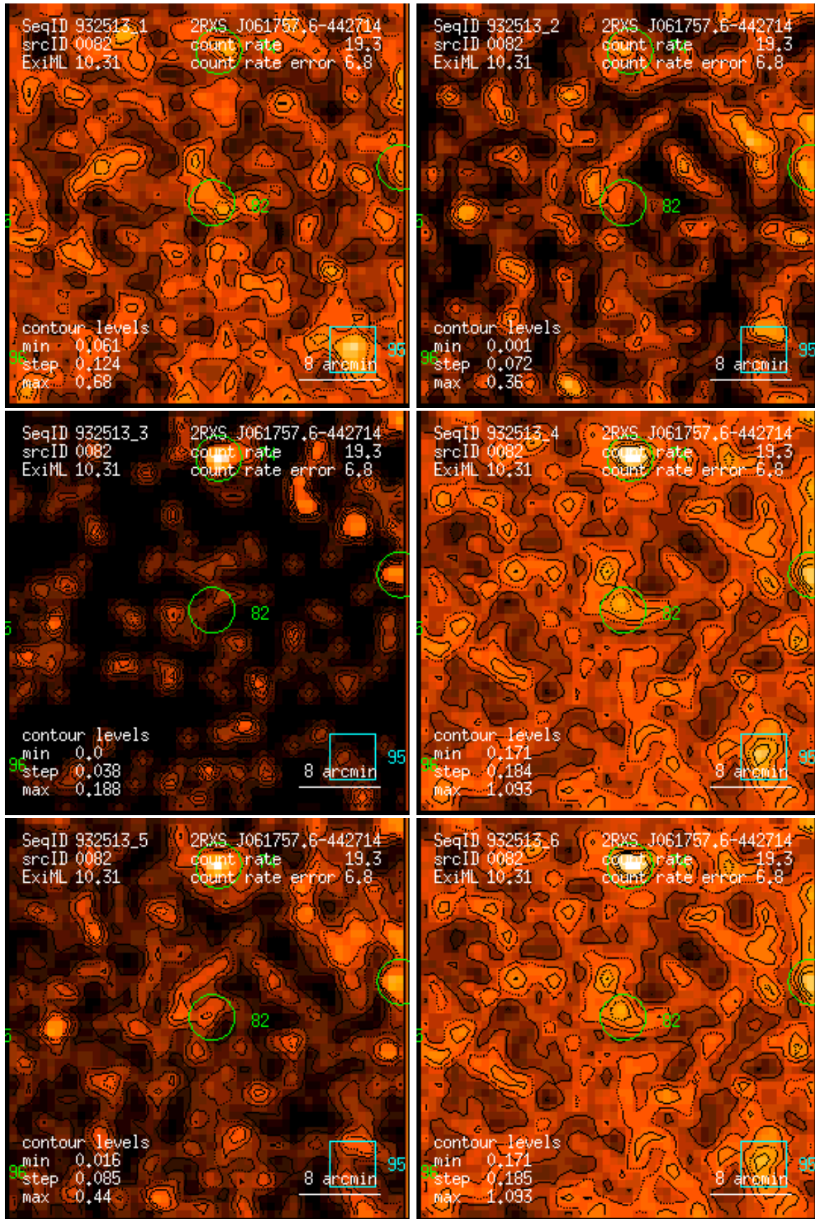
Figure 82: RASS 932513: detection 0082: band rate images, Gaussian filter: (1) PSPC channels 11 – 41, (2) 52 – 90, (3) 91 – 201, (4) 11 – 235, (5) 52 – 201, (6) 11 – 201. Broad band rates in counts/ks. Band rate contour levels in counts/ks/arcmin 2 .
