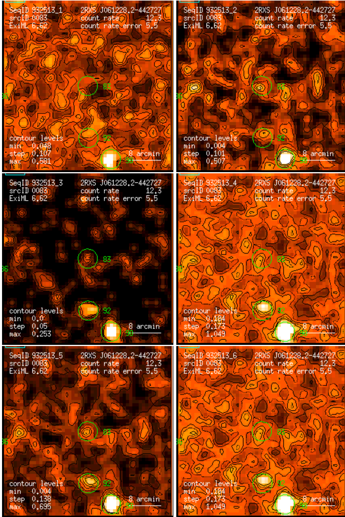
Figure 83: RASS 932513: detection 0083: band rate images, Gaussian filter: (1) PSPC channels 11 – 41, (2) 52 – 90, (3) 91 – 201, (4) 11 – 235, (5) 52 – 201, (6) 11 – 201. Broad band rates in counts/ks. Band rate contour levels in counts/ks/arcmin 2 .
