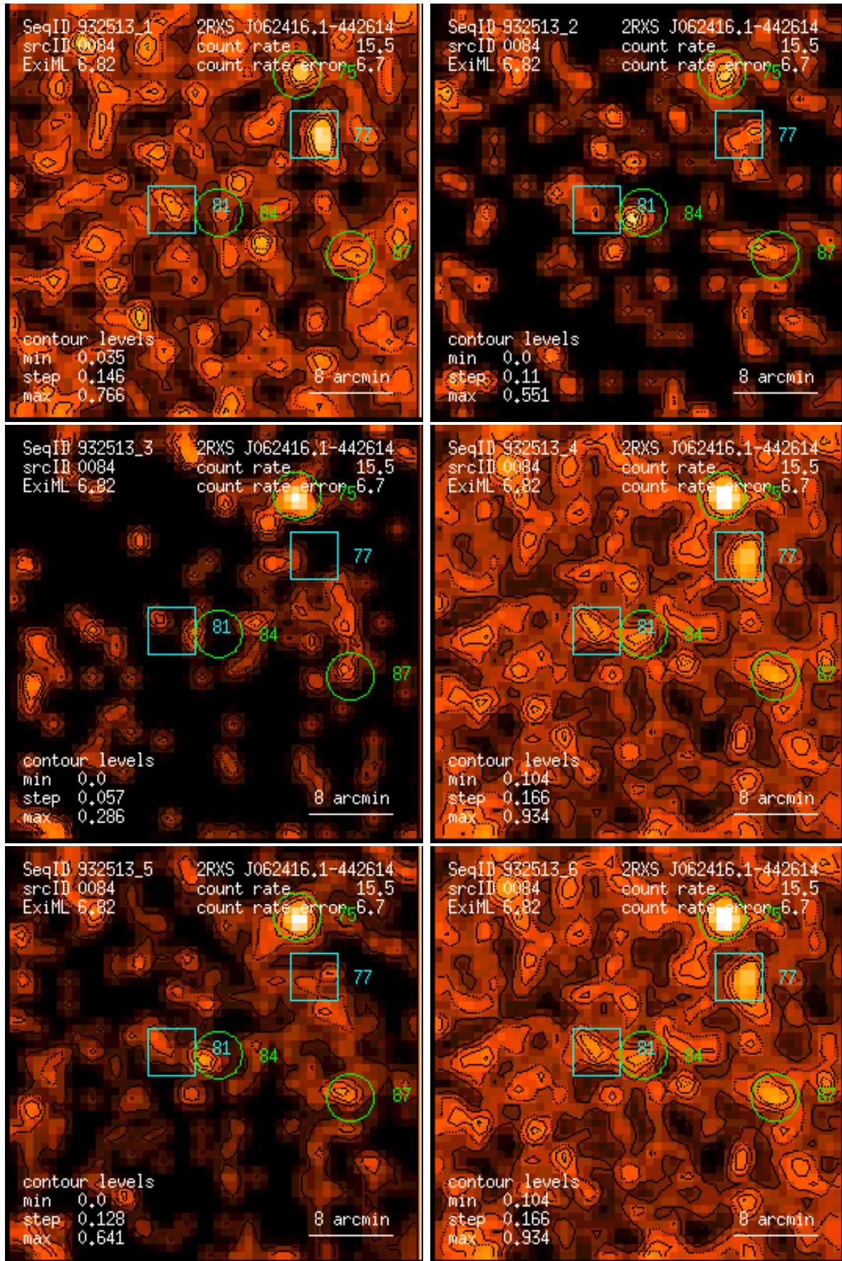
Figure 84: RASS 932513: detection 0084: band rate images, Gaussian filter: (1) PSPC channels 11 – 41, (2) 52 – 90, (3) 91 – 201, (4) 11 – 235, (5) 52 – 201, (6) 11 – 201. Broad band rates in counts/ks. Band rate contour levels in counts/ks/arcmin 2 .
