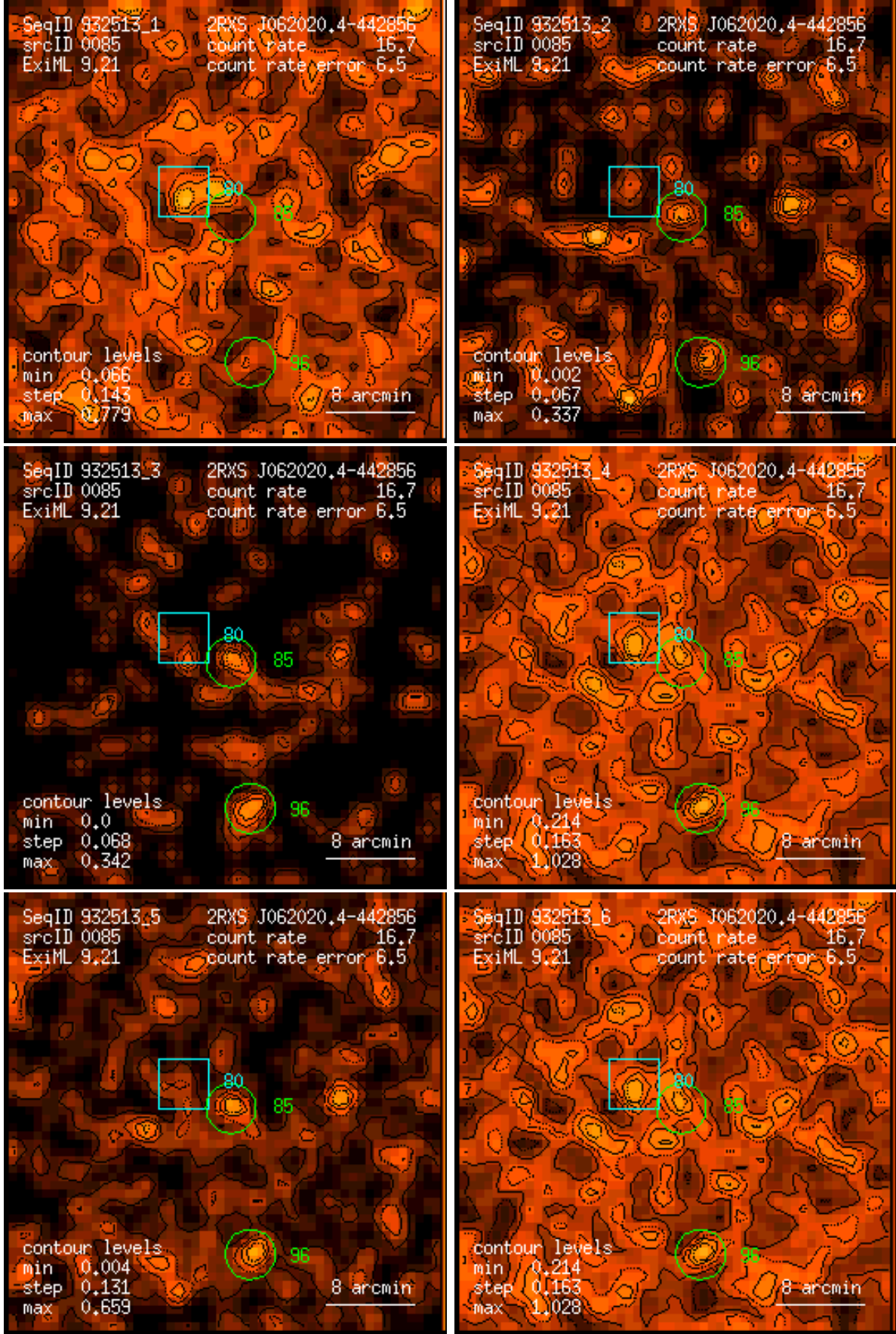
Figure 85: RASS 932513: detection 0085: band rate images, Gaussian filter: (1) PSPC channels 11 – 41, (2) 52 – 90, (3) 91 – 201, (4) 11 – 235, (5) 52 – 201, (6) 11 – 201. Broad band rates in counts/ks. Band rate contour levels in counts/ks/arcmin 2 .
