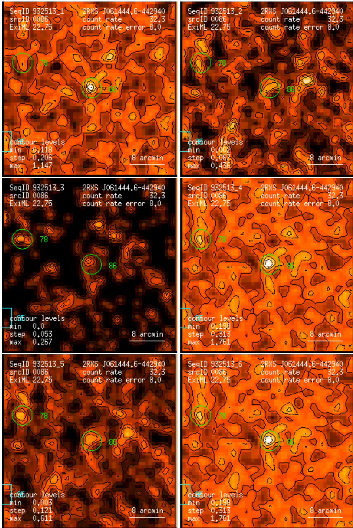
Figure 86: RASS 932513: detection 0086: band rate images, Gaussian filter: (1) PSPC channels 11 – 41, (2) 52 – 90, (3) 91 – 201, (4) 11 – 235, (5) 52 – 201, (6) 11 – 201. Broad band rates in counts/ks. Band rate contour levels in counts/ks/arcmin 2 .
