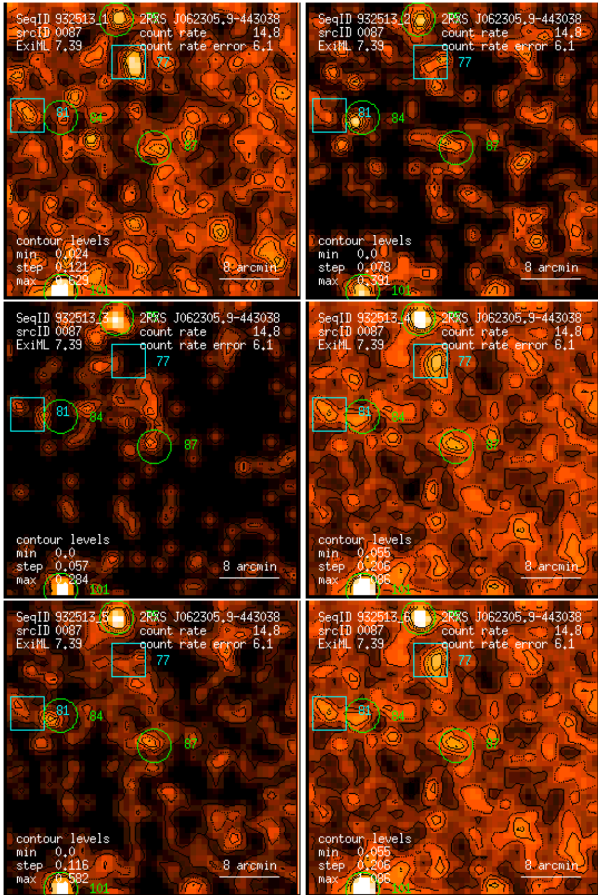
Figure 87: RASS 932513: detection 0087: band rate images, Gaussian filter: (1) PSPC channels 11 – 41, (2) 52 – 90, (3) 91 – 201, (4) 11 – 235, (5) 52 – 201, (6) 11 – 201. Broad band rates in counts/ks. Band rate contour levels in counts/ks/arcmin 2 .
