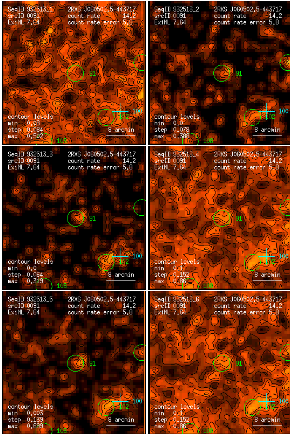
Figure 91: RASS 932513: detection 0091: band rate images, Gaussian filter: (1) PSPC channels 11 – 41, (2) 52 – 90, (3) 91 – 201, (4) 11 – 235, (5) 52 – 201, (6) 11 – 201. Broad band rates in counts/ks. Band rate contour levels in counts/ks/arcmin 2 .
