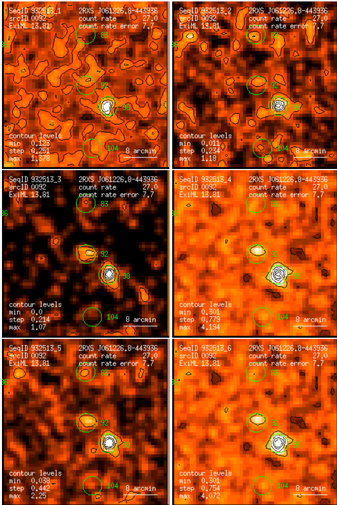
Figure 92: RASS 932513: detection 0092: band rate images, Gaussian filter: (1) PSPC channels 11 – 41, (2) 52 – 90, (3) 91 – 201, (4) 11 – 235, (5) 52 – 201, (6) 11 – 201. Broad band rates in counts/ks. Band rate contour levels in counts/ks/arcmin 2 .
