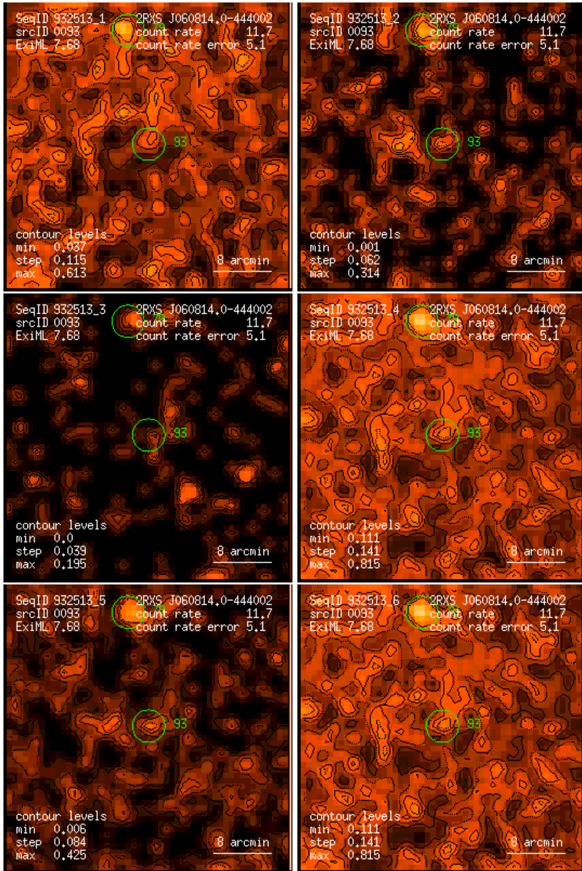
Figure 93: RASS 932513: detection 0093: band rate images, Gaussian filter: (1) PSPC channels 11 – 41, (2) 52 – 90, (3) 91 – 201, (4) 11 – 235, (5) 52 – 201, (6) 11 – 201. Broad band rates in counts/ks. Band rate contour levels in counts/ks/arcmin 2 .
