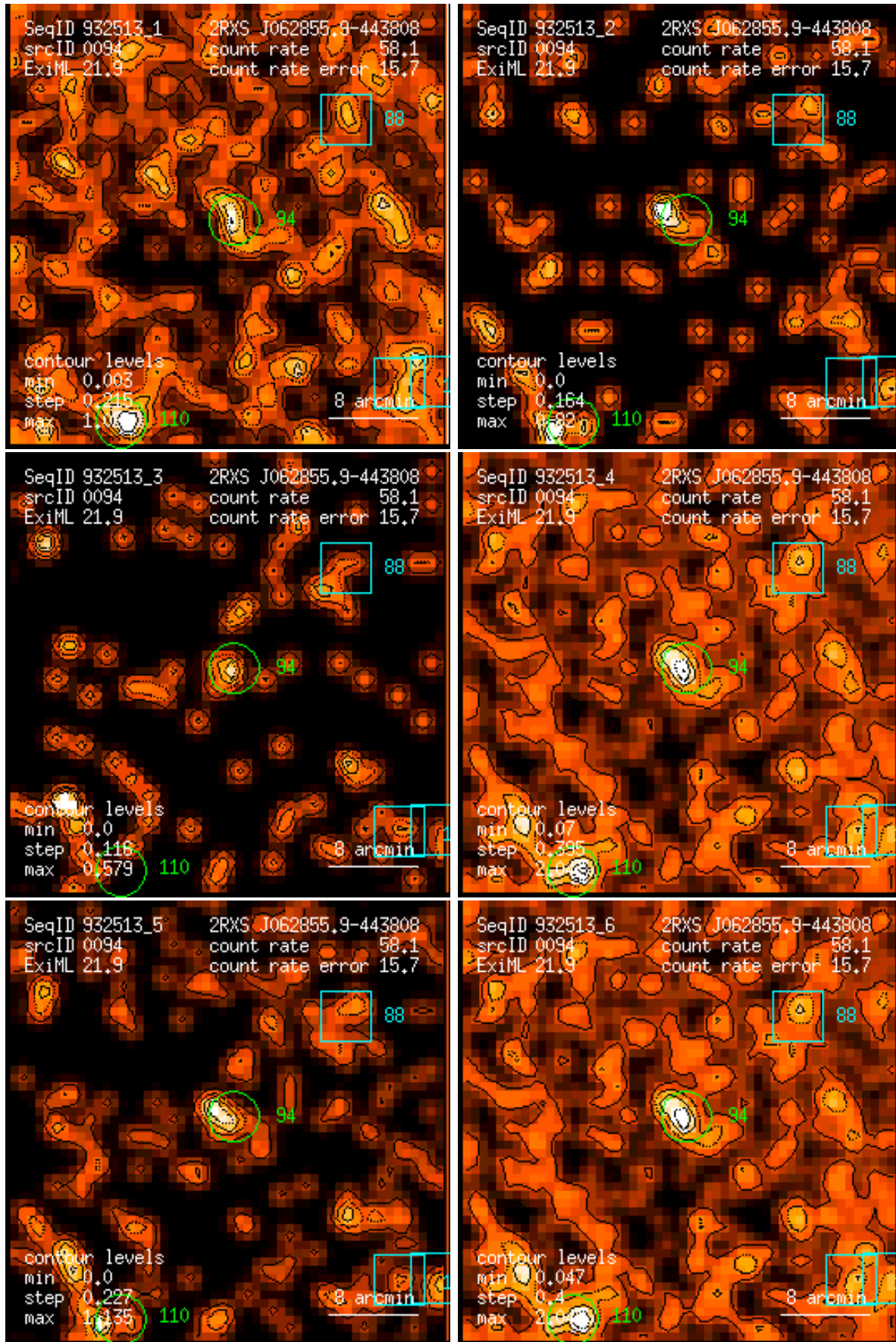
Figure 94: RASS 932513: detection 0094: band rate images, Gaussian filter: (1) PSPC channels 11 – 41, (2) 52 – 90, (3) 91 – 201, (4) 11 – 235, (5) 52 – 201, (6) 11 – 201. Broad band rates in counts/ks. Band rate contour levels in counts/ks/arcmin 2 .
