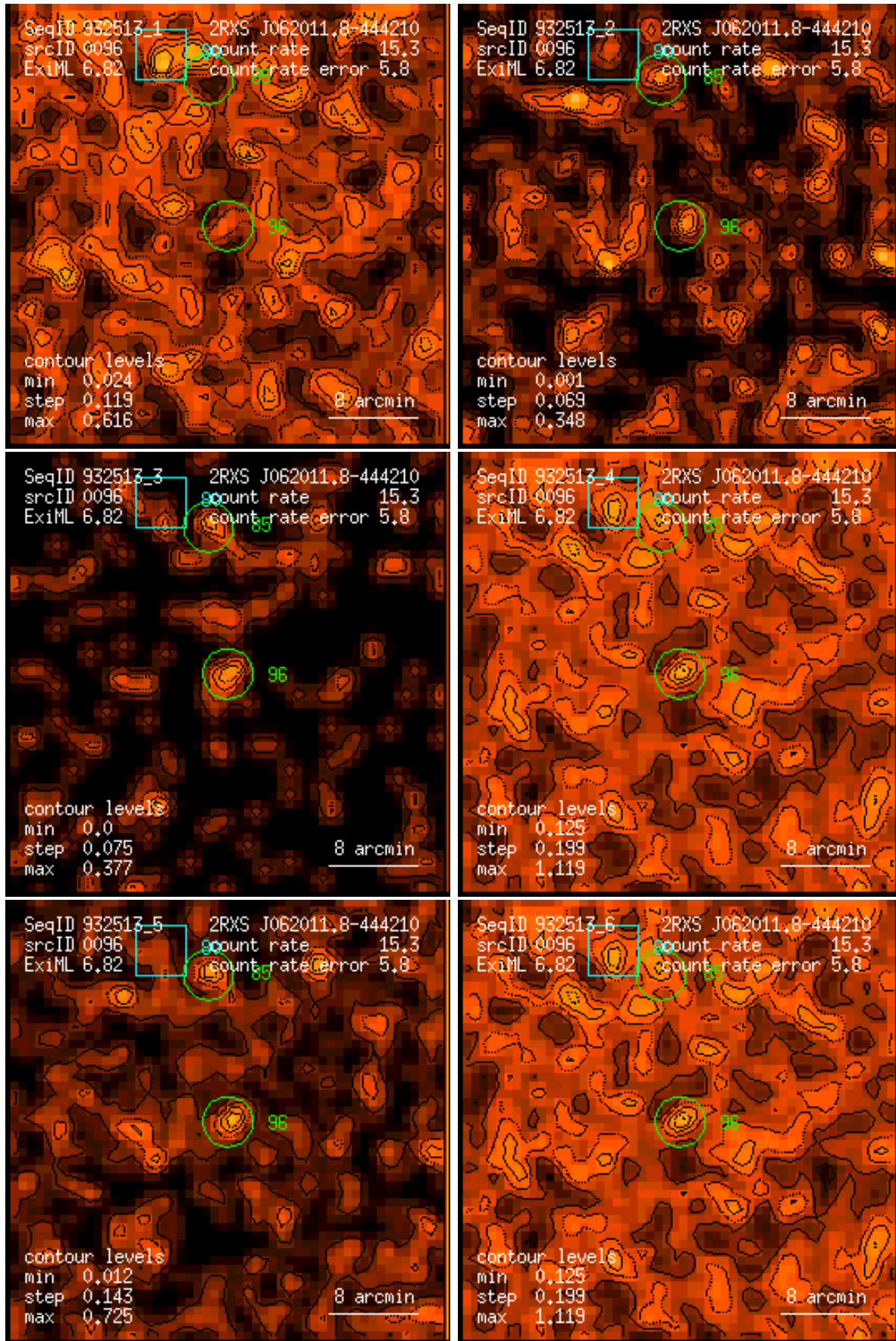
Figure 96: RASS 932513: detection 0096: band rate images, Gaussian filter: (1) PSPC channels 11 – 41, (2) 52 – 90, (3) 91 – 201, (4) 11 – 235, (5) 52 – 201, (6) 11 – 201. Broad band rates in counts/ks. Band rate contour levels in counts/ks/arcmin 2 .
