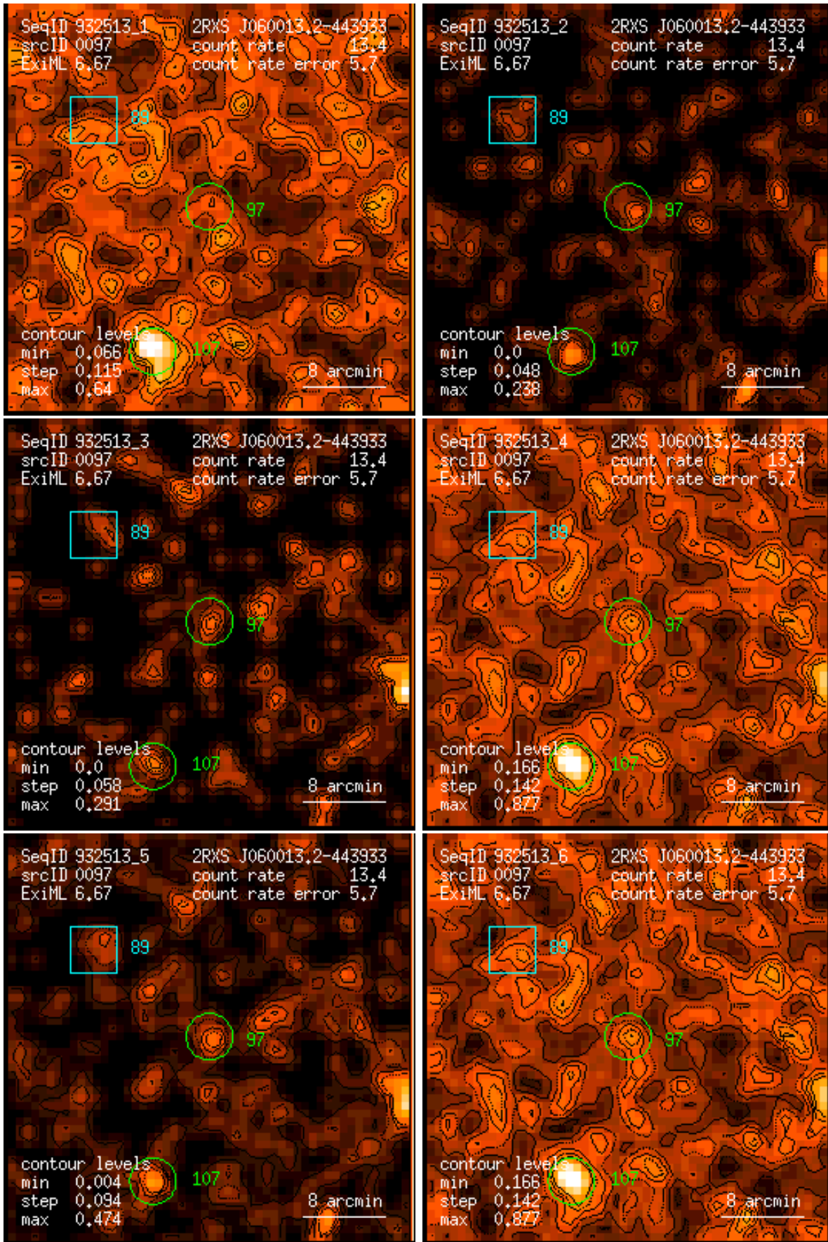
Figure 97: RASS 932513: detection 0097: band rate images, Gaussian filter: (1) PSPC channels 11 – 41, (2) 52 – 90, (3) 91 – 201, (4) 11 – 235, (5) 52 – 201, (6) 11 – 201. Broad band rates in counts/ks. Band rate contour levels in counts/ks/arcmin 2 .
