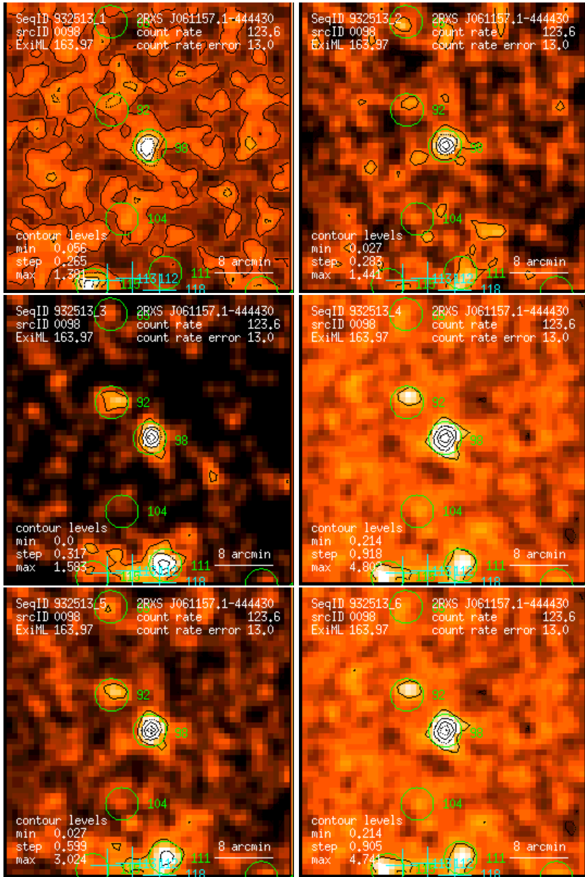
Figure 98: RASS 932513: detection 0098: band rate images, Gaussian filter: (1) PSPC channels 11 – 41, (2) 52 – 90, (3) 91 – 201, (4) 11 – 235, (5) 52 – 201, (6) 11 – 201. Broad band rates in counts/ks. Band rate contour levels in counts/ks/arcmin 2 .
