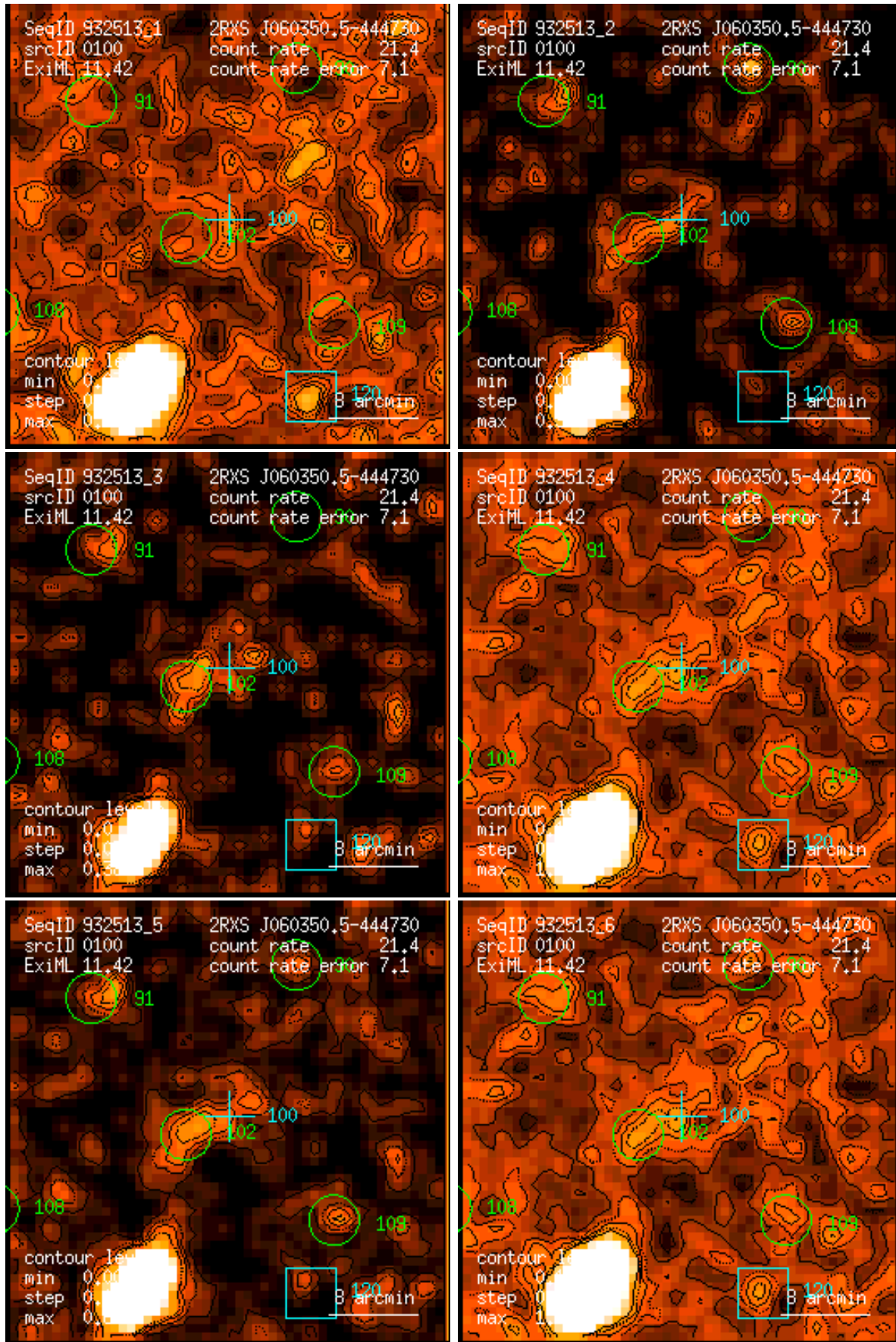
Figure 100: RASS 932513: detection 0100: band rate images, Gaussian filter: (1) PSPC channels 11 – 41, (2) 52 – 90, (3) 91 – 201, (4) 11 – 235, (5) 52 – 201, (6) 11 – 201. Broad band rates in counts/ks. Band rate contour levels in counts/ks/arcmin 2 .
