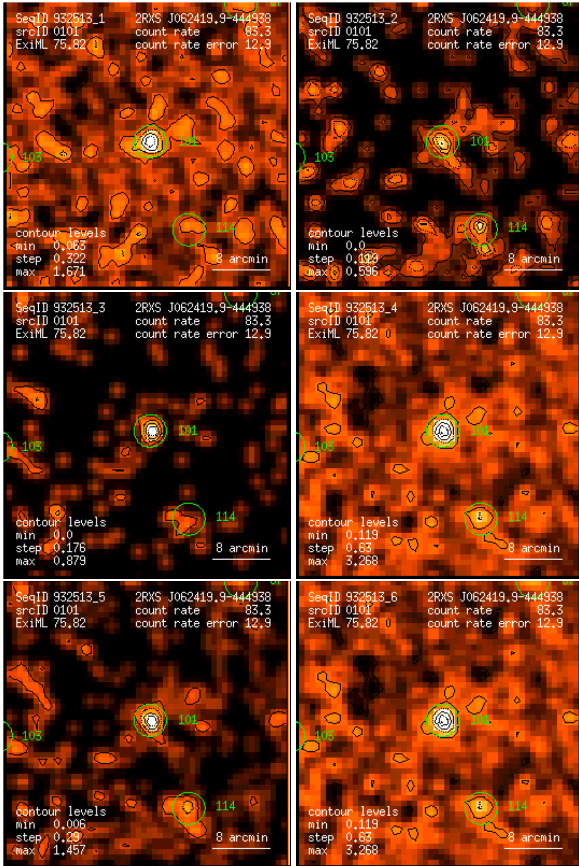
Figure 101: RASS 932513: detection 0101: band rate images, Gaussian filter: (1) PSPC channels 11 – 41, (2) 52 – 90, (3) 91 – 201, (4) 11 – 235, (5) 52 – 201, (6) 11 – 201. Broad band rates in counts/ks. Band rate contour levels in counts/ks/arcmin 2 .
