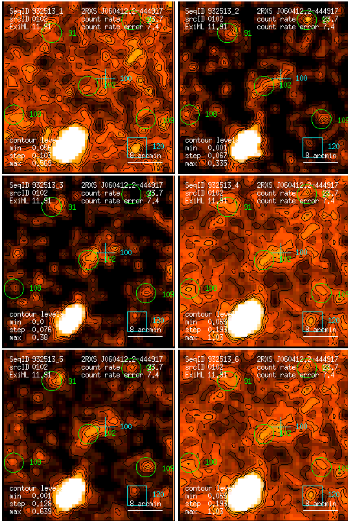
Figure 102: RASS 932513: detection 0102: band rate images, Gaussian filter: (1) PSPC channels 11 – 41, (2) 52 – 90, (3) 91 – 201, (4) 11 – 235, (5) 52 – 201, (6) 11 – 201. Broad band rates in counts/ks. Band rate contour levels in counts/ks/arcmin 2 .
