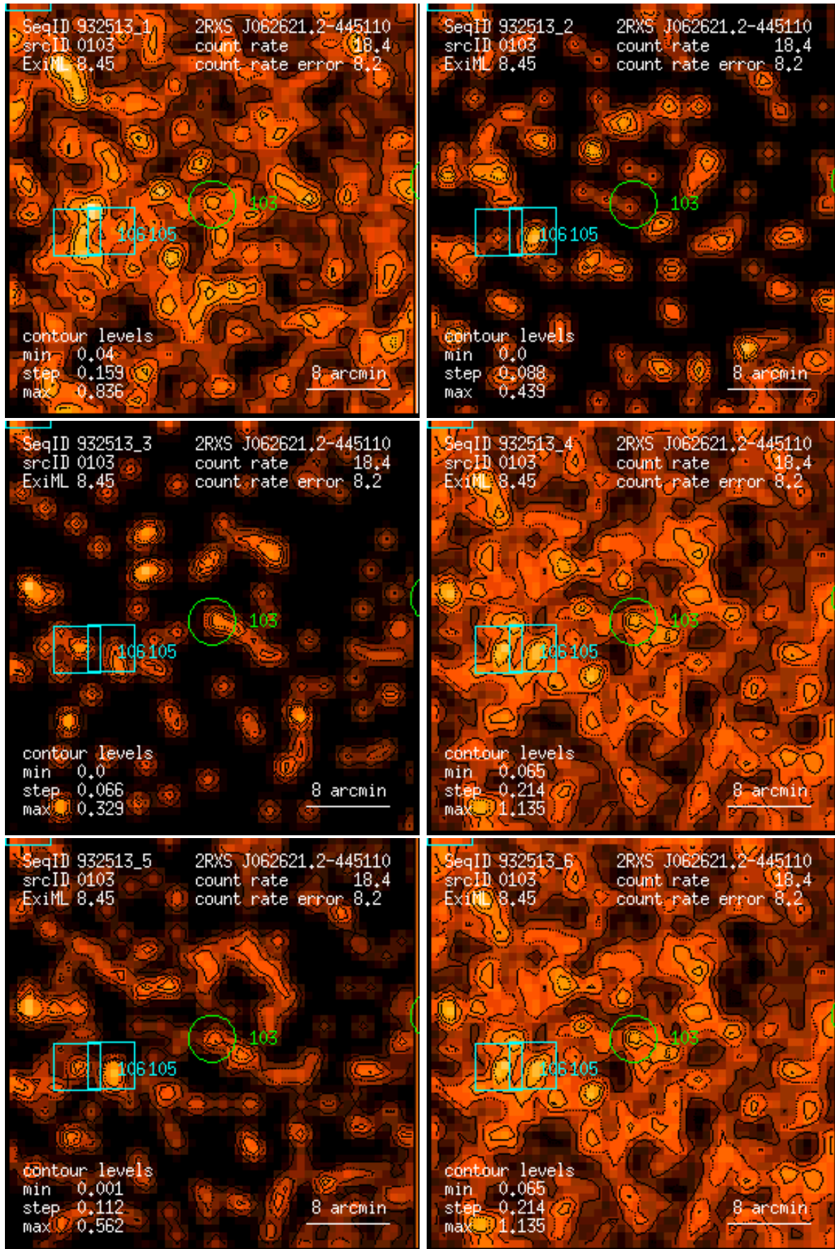
Figure 103: RASS 932513: detection 0103: band rate images, Gaussian filter: (1) PSPC channels 11 – 41, (2) 52 – 90, (3) 91 – 201, (4) 11 – 235, (5) 52 – 201, (6) 11 – 201. Broad band rates in counts/ks. Band rate contour levels in counts/ks/arcmin 2 .
