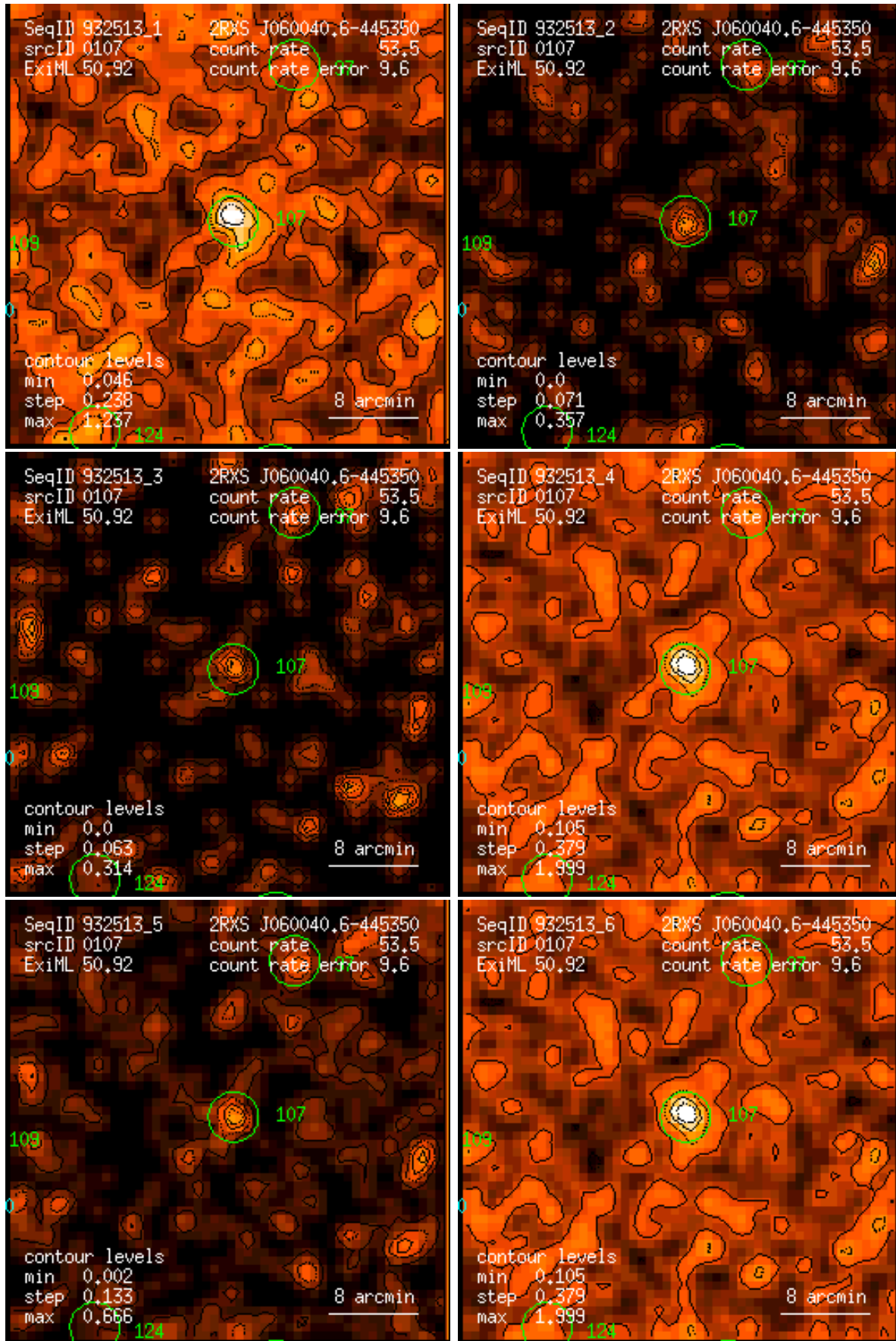
Figure 107: RASS 932513: detection 0107: band rate images, Gaussian filter: (1) PSPC channels 11 – 41, (2) 52 – 90, (3) 91 – 201, (4) 11 – 235, (5) 52 – 201, (6) 11 – 201. Broad band rates in counts/ks. Band rate contour levels in counts/ks/arcmin 2 .
