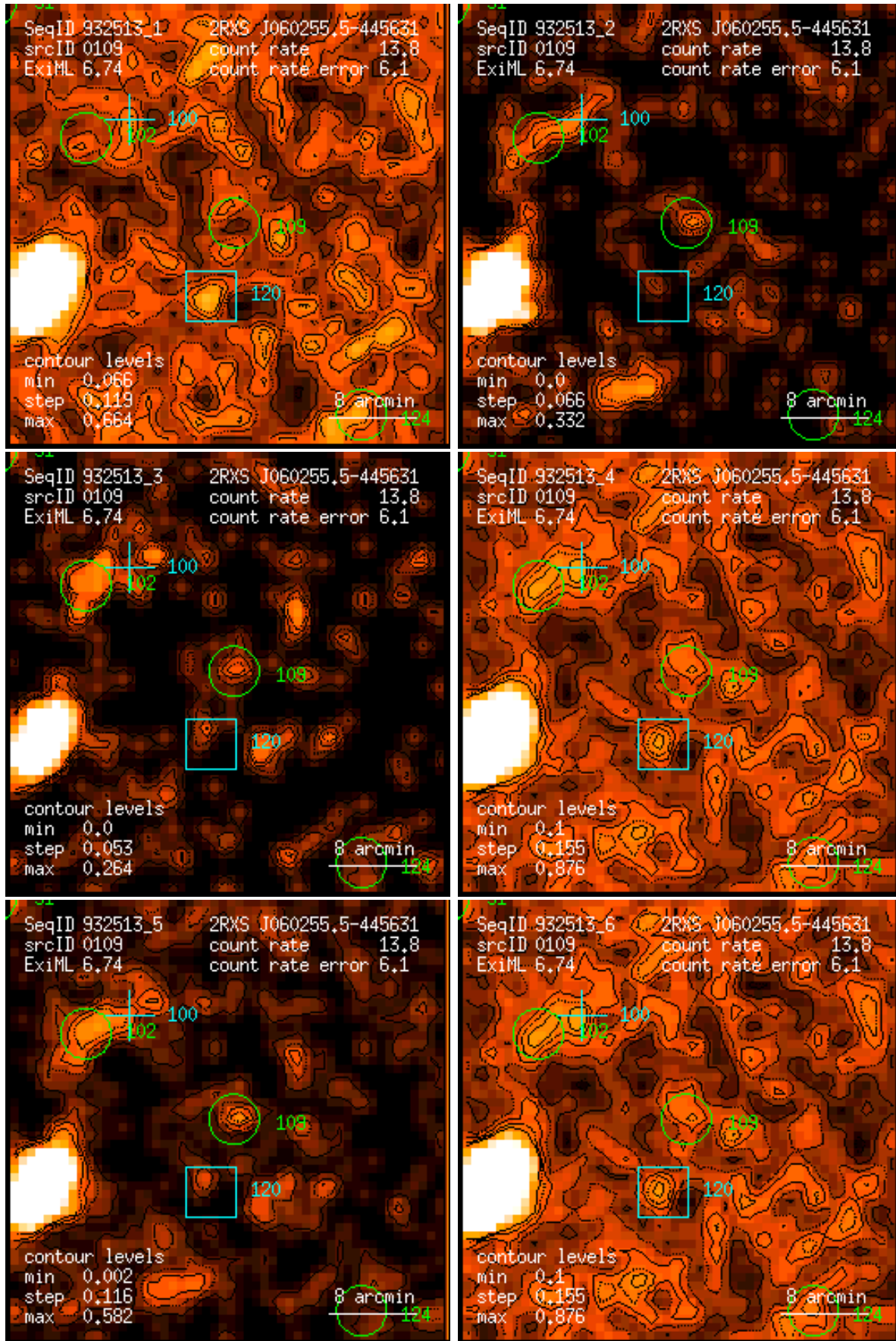
Figure 109: RASS 932513: detection 0109: band rate images, Gaussian filter: (1) PSPC channels 11 – 41, (2) 52 – 90, (3) 91 – 201, (4) 11 – 235, (5) 52 – 201, (6) 11 – 201. Broad band rates in counts/ks. Band rate contour levels in counts/ks/arcmin 2 .
