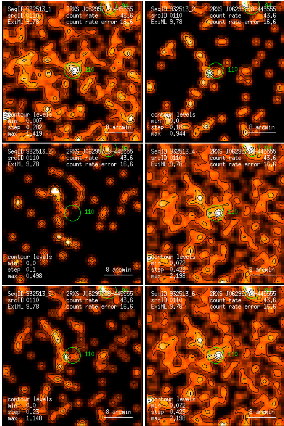
Figure 110: RASS 932513: detection 0110: band rate images, Gaussian filter: (1) PSPC channels 11 – 41, (2) 52 – 90, (3) 91 – 201, (4) 11 – 235, (5) 52 – 201, (6) 11 – 201. Broad band rates in counts/ks. Band rate contour levels in counts/ks/arcmin 2 .
