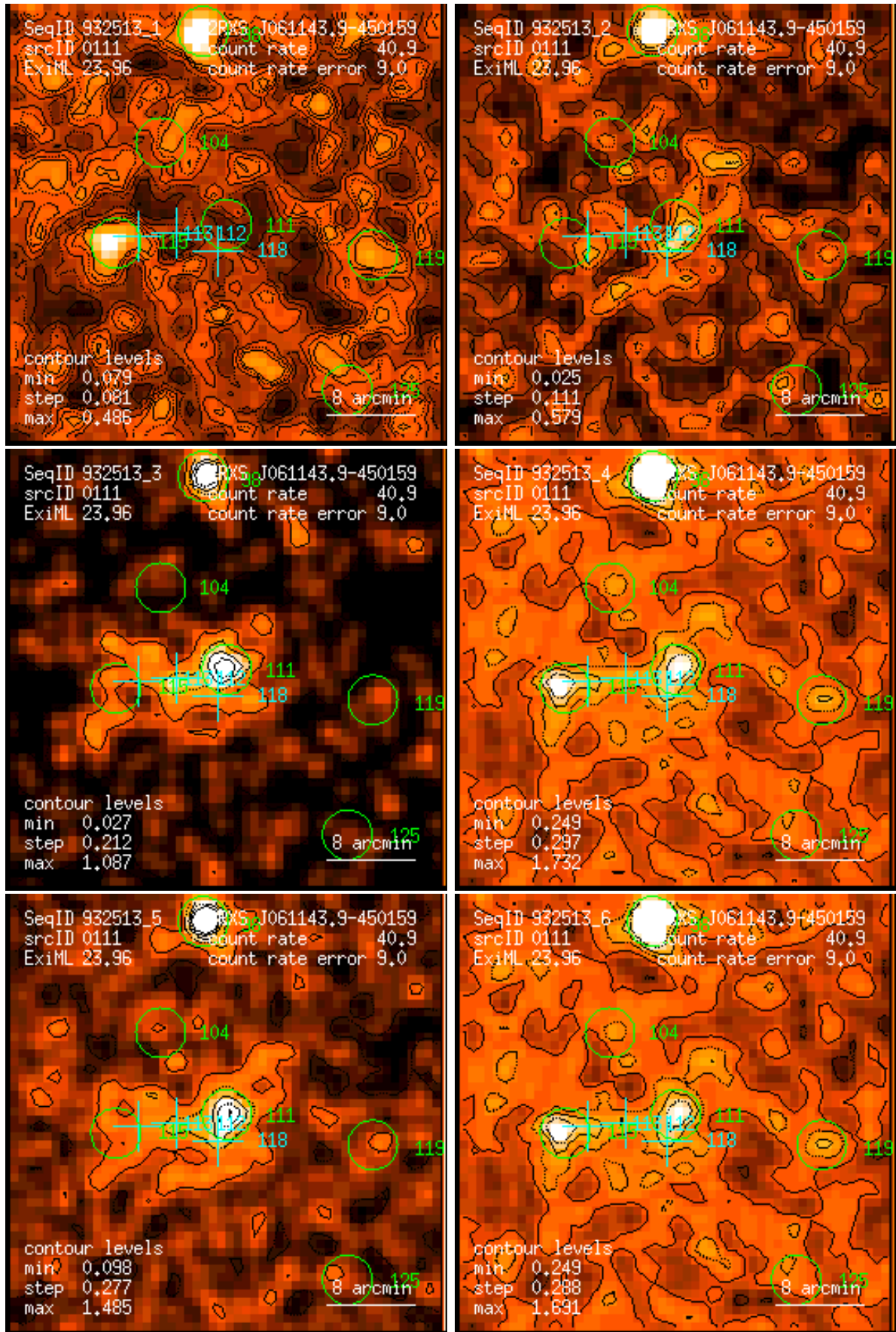
Figure 111: RASS 932513: detection 0111: band rate images, Gaussian filter: (1) PSPC channels 11 – 41, (2) 52 – 90, (3) 91 – 201, (4) 11 – 235, (5) 52 – 201, (6) 11 – 201. Broad band rates in counts/ks. Band rate contour levels in counts/ks/arcmin 2 .
