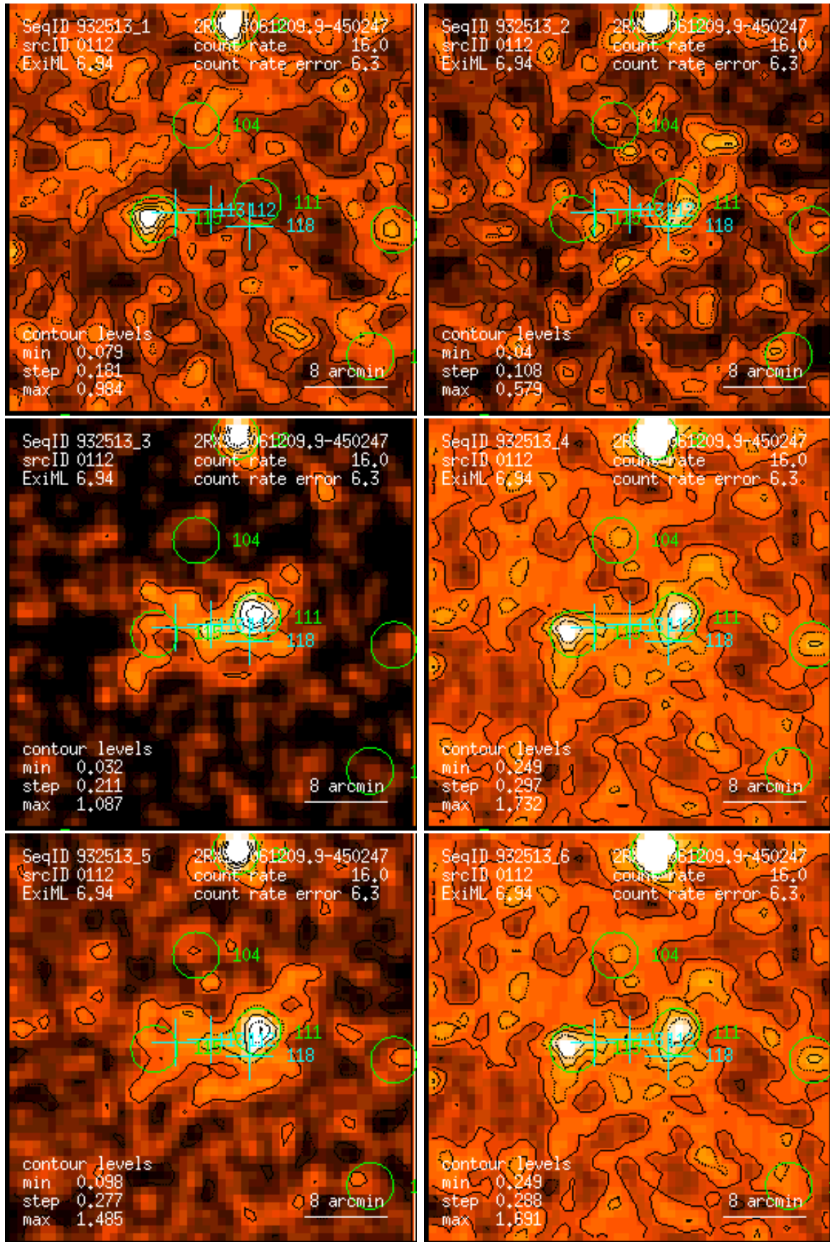
Figure 112: RASS 932513: detection 0112: band rate images, Gaussian filter: (1) PSPC channels 11 – 41, (2) 52 – 90, (3) 91 – 201, (4) 11 – 235, (5) 52 – 201, (6) 11 – 201. Broad band rates in counts/ks. Band rate contour levels in counts/ks/arcmin 2 .
