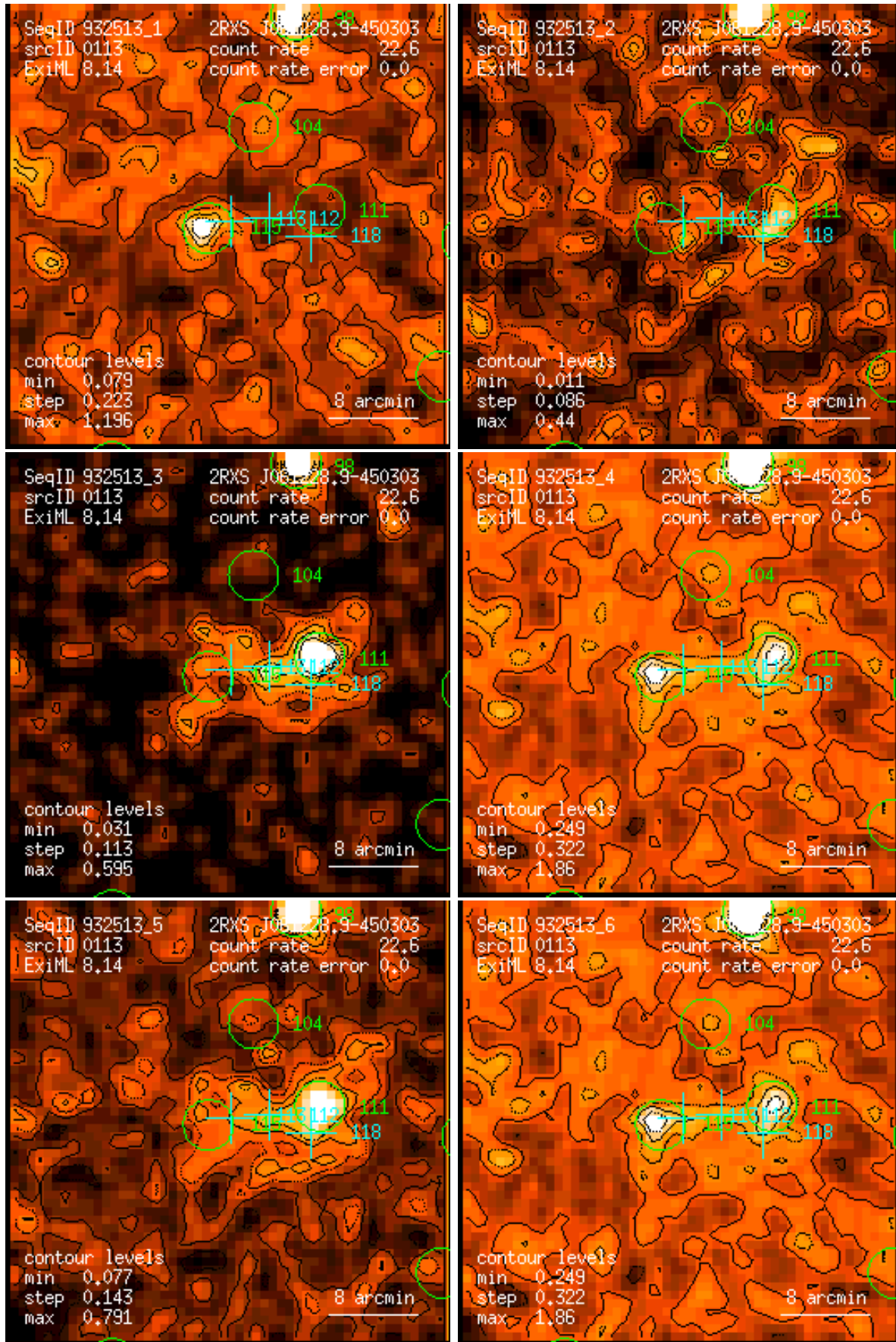
Figure 113: RASS 932513: detection 0113: band rate images, Gaussian filter: (1) PSPC channels 11 – 41, (2) 52 – 90, (3) 91 – 201, (4) 11 – 235, (5) 52 – 201, (6) 11 – 201. Broad band rates in counts/ks. Band rate contour levels in counts/ks/arcmin 2 .
