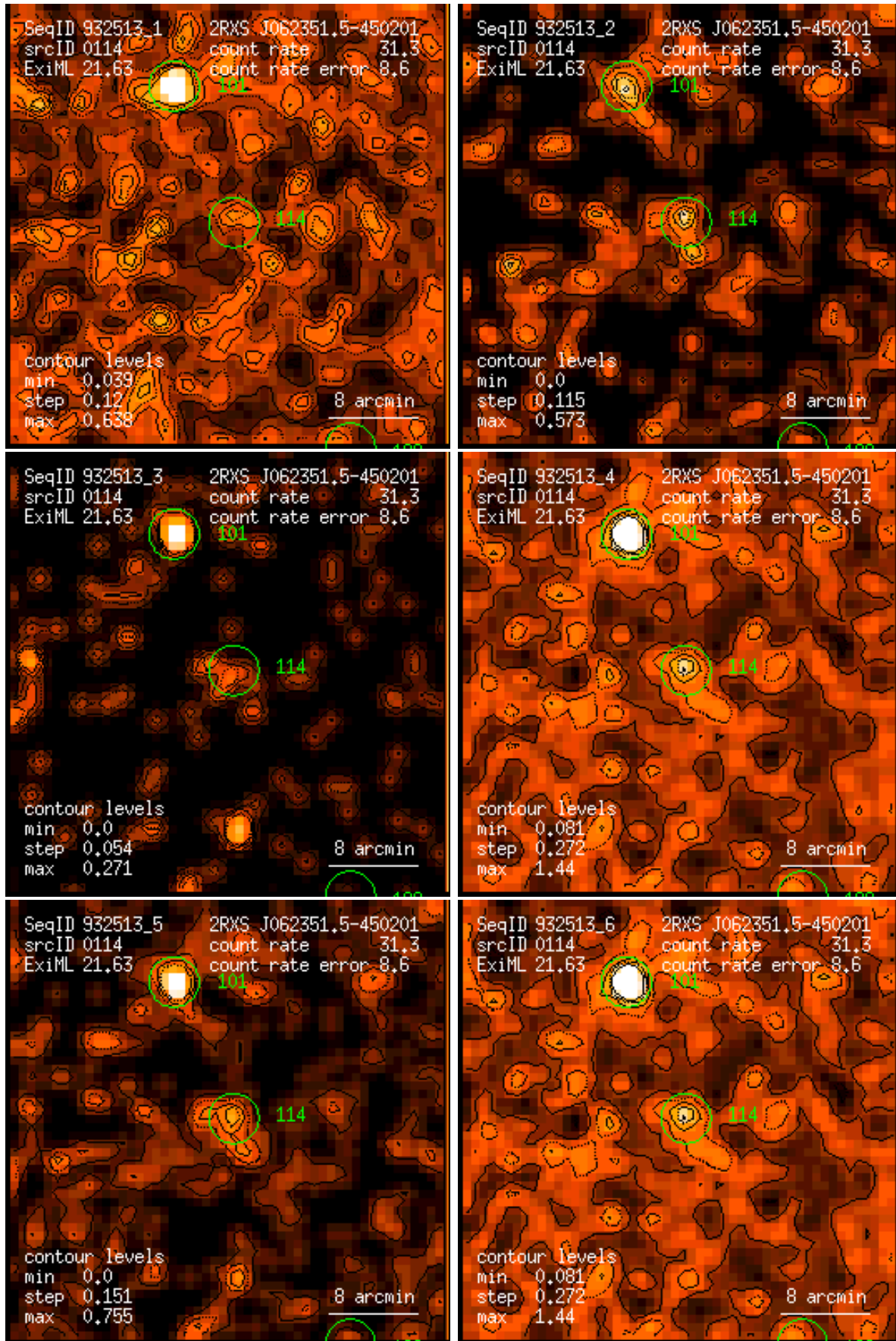
Figure 114: RASS 932513: detection 0114: band rate images, Gaussian filter: (1) PSPC channels 11 – 41, (2) 52 – 90, (3) 91 – 201, (4) 11 – 235, (5) 52 – 201, (6) 11 – 201. Broad band rates in counts/ks. Band rate contour levels in counts/ks/arcmin 2 .
