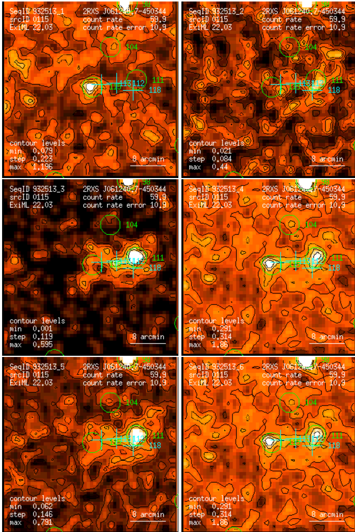
Figure 115: RASS 932513: detection 0115: band rate images, Gaussian filter: (1) PSPC channels 11 – 41, (2) 52 – 90, (3) 91 – 201, (4) 11 – 235, (5) 52 – 201, (6) 11 – 201. Broad band rates in counts/ks. Band rate contour levels in counts/ks/arcmin 2 .
