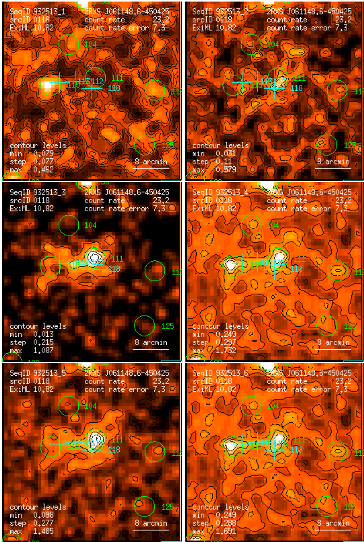
Figure 118: RASS 932513: detection 0118: band rate images, Gaussian filter: (1) PSPC channels 11 – 41, (2) 52 – 90, (3) 91 – 201, (4) 11 – 235, (5) 52 – 201, (6) 11 – 201. Broad band rates in counts/ks. Band rate contour levels in counts/ks/arcmin 2 .
