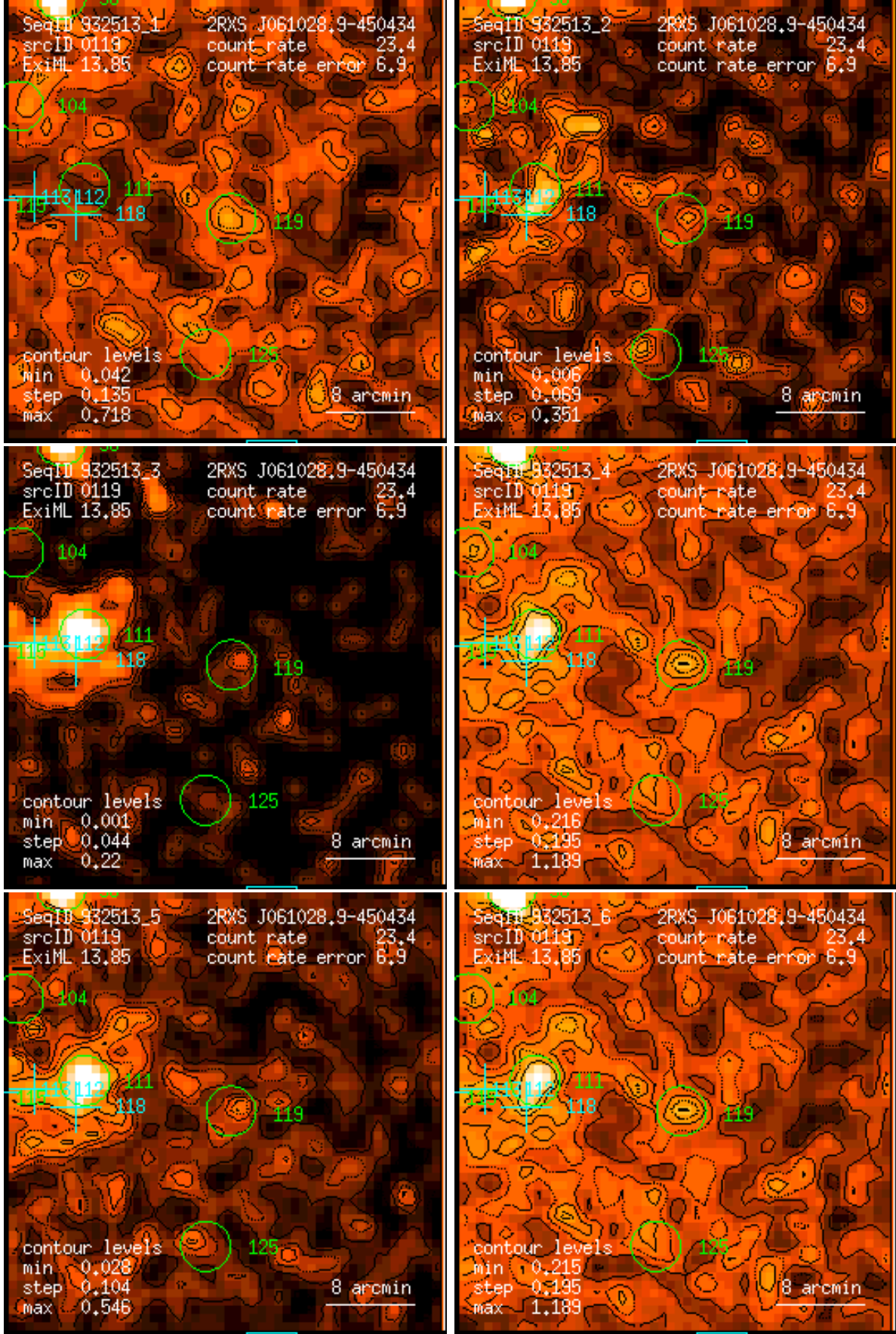
Figure 119: RASS 932513: detection 0119: band rate images, Gaussian filter: (1) PSPC channels 11 – 41, (2) 52 – 90, (3) 91 – 201, (4) 11 – 235, (5) 52 – 201, (6) 11 – 201. Broad band rates in counts/ks. Band rate contour levels in counts/ks/arcmin 2 .
