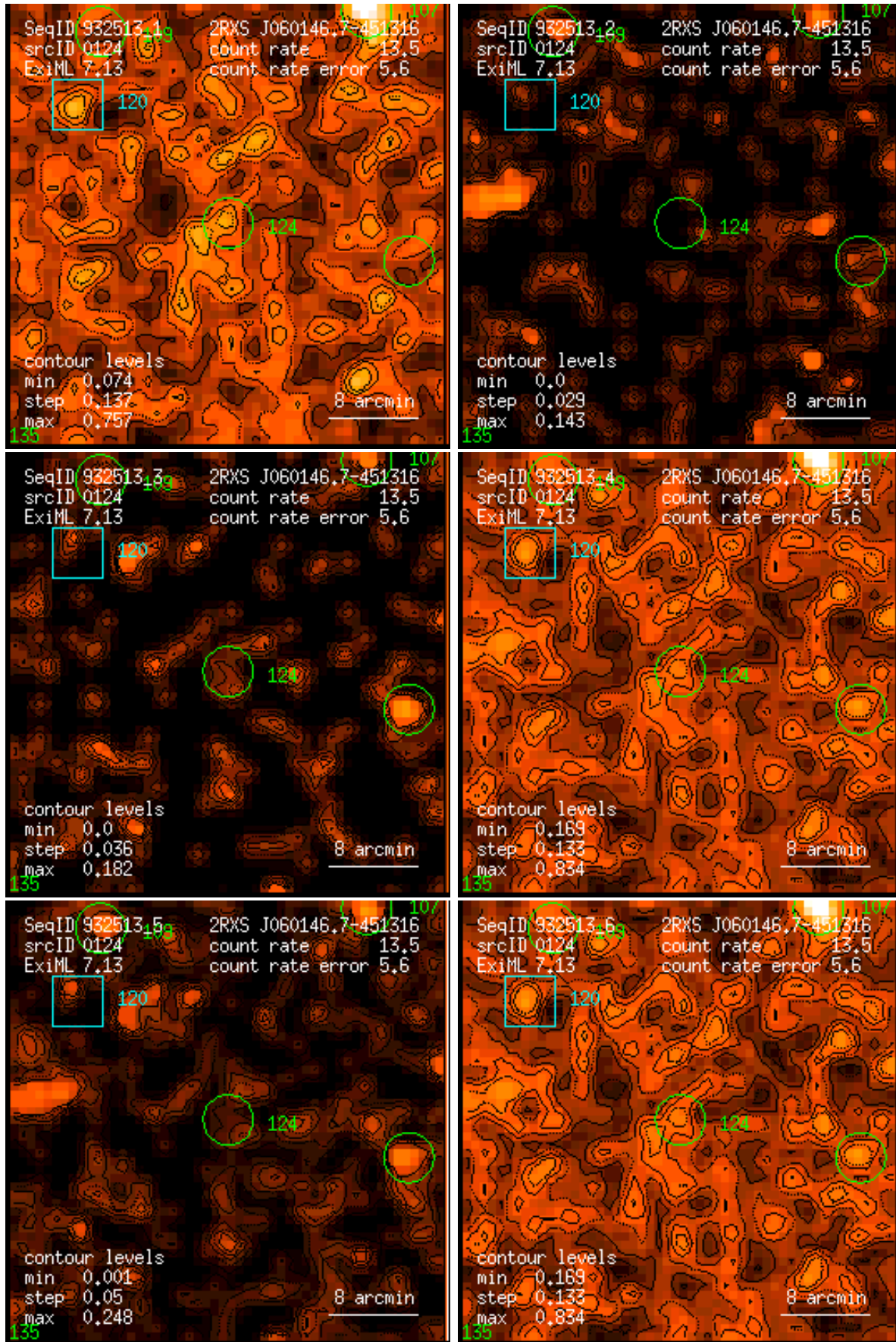
Figure 124: RASS 932513: detection 0124: band rate images, Gaussian filter: (1) PSPC channels 11 – 41, (2) 52 – 90, (3) 91 – 201, (4) 11 – 235, (5) 52 – 201, (6) 11 – 201. Broad band rates in counts/ks. Band rate contour levels in counts/ks/arcmin 2 .
