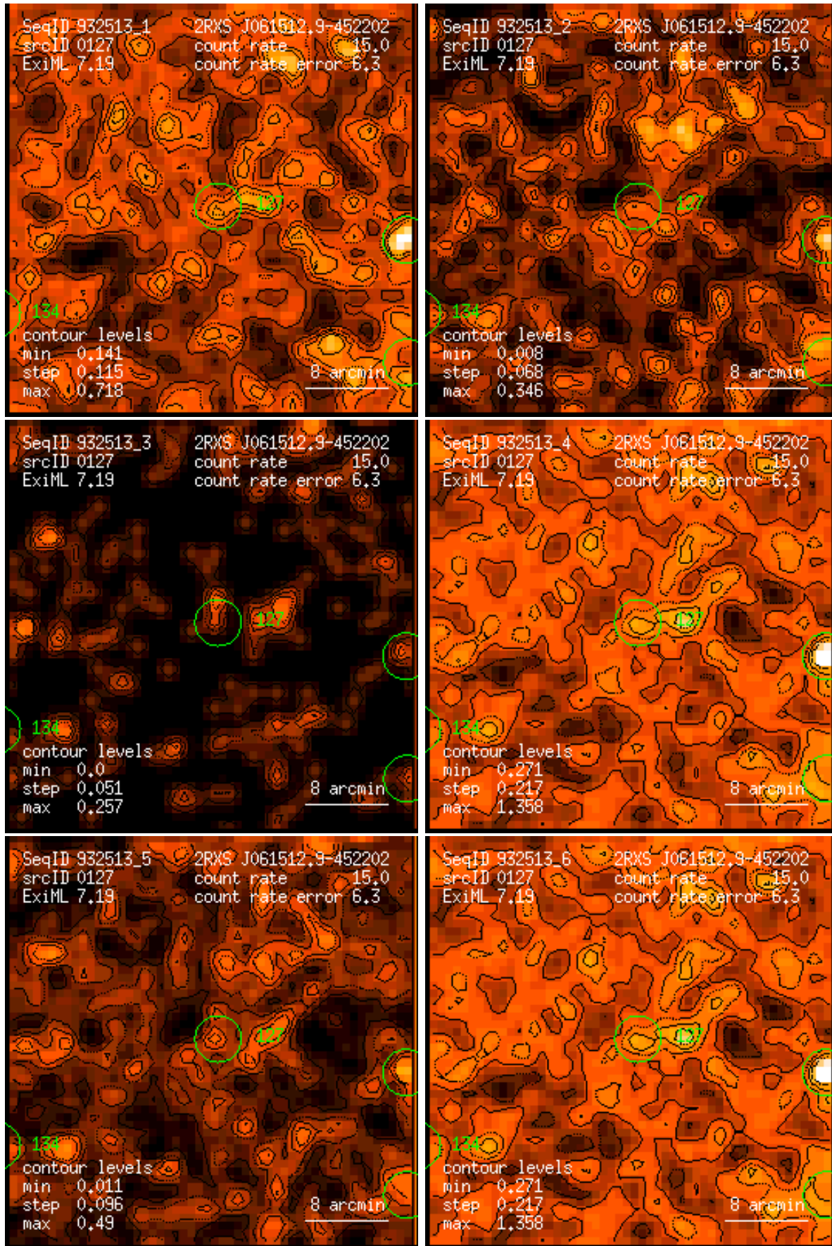
Figure 127: RASS 932513: detection 0127: band rate images, Gaussian filter: (1) PSPC channels 11 – 41, (2) 52 – 90, (3) 91 – 201, (4) 11 – 235, (5) 52 – 201, (6) 11 – 201. Broad band rates in counts/ks. Band rate contour levels in counts/ks/arcmin 2 .
