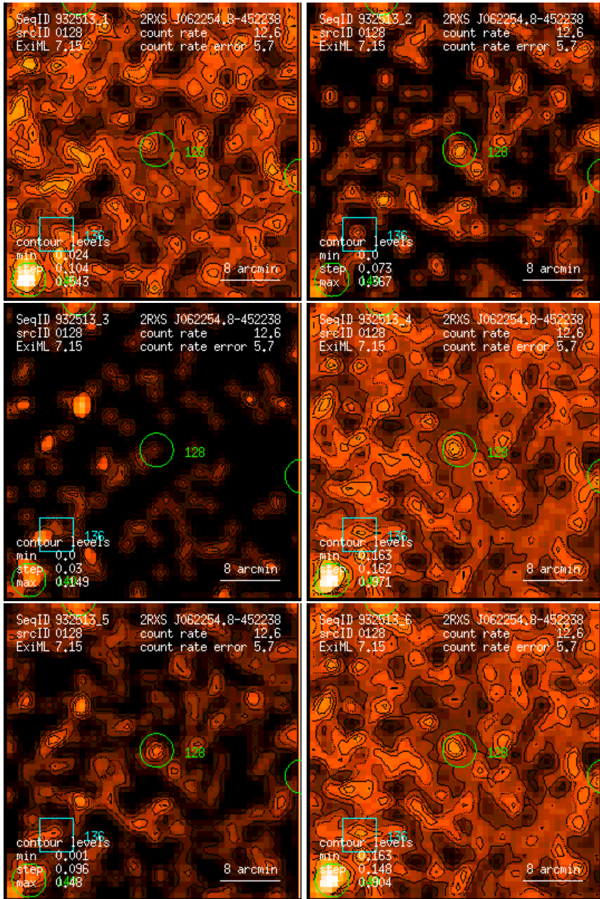
Figure 128: RASS 932513: detection 0128: band rate images, Gaussian filter: (1) PSPC channels 11 – 41, (2) 52 – 90, (3) 91 – 201, (4) 11 – 235, (5) 52 – 201, (6) 11 – 201. Broad band rates in counts/ks. Band rate contour levels in counts/ks/arcmin 2 .
