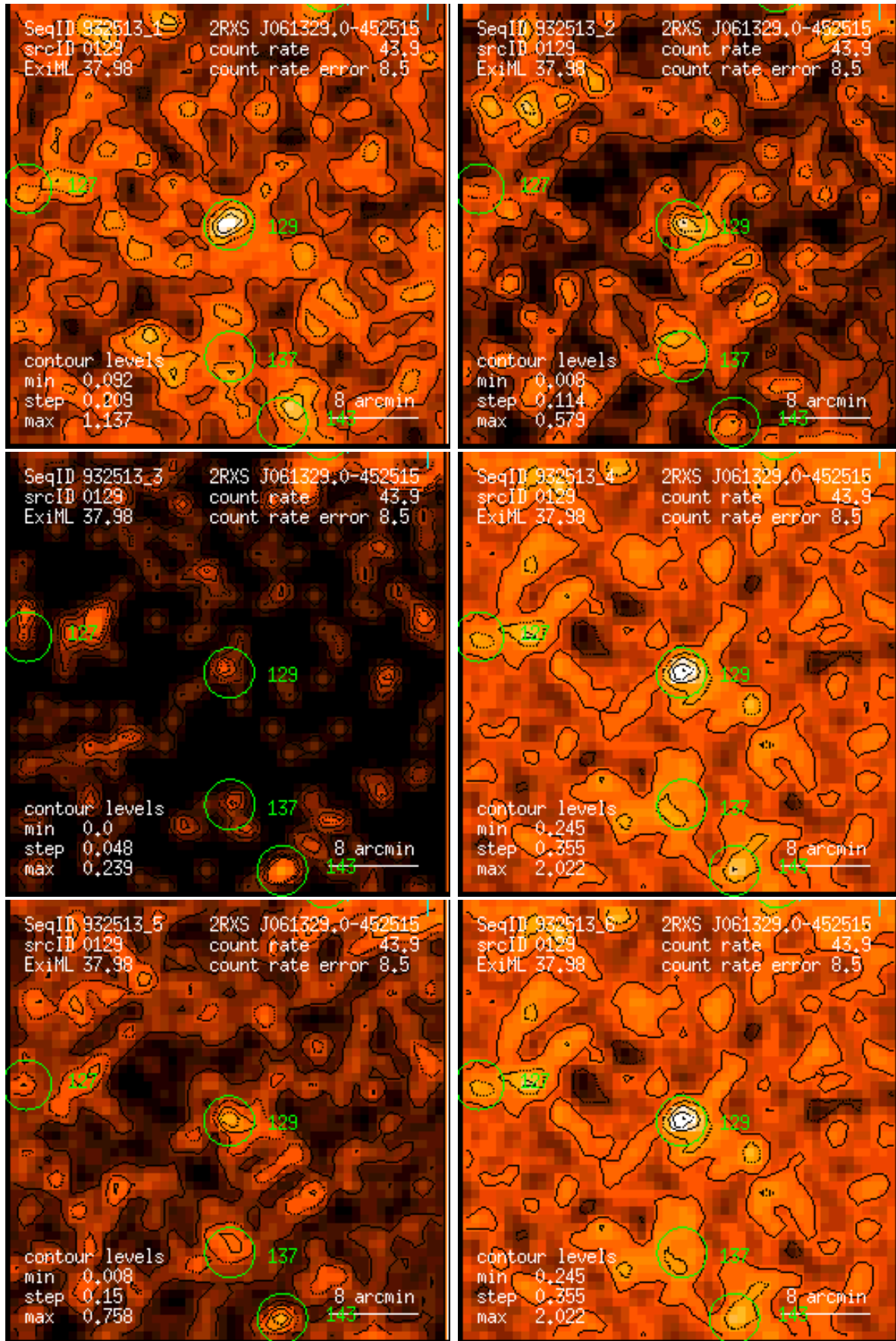
Figure 129: RASS 932513: detection 0129: band rate images, Gaussian filter: (1) PSPC channels 11 – 41, (2) 52 – 90, (3) 91 – 201, (4) 11 – 235, (5) 52 – 201, (6) 11 – 201. Broad band rates in counts/ks. Band rate contour levels in counts/ks/arcmin 2 .
