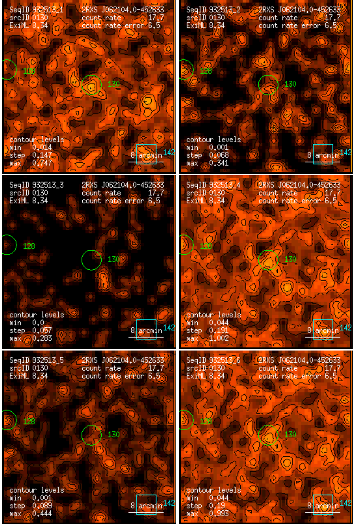
Figure 130: RASS 932513: detection 0130: band rate images, Gaussian filter: (1) PSPC channels 11 – 41, (2) 52 – 90, (3) 91 – 201, (4) 11 – 235, (5) 52 – 201, (6) 11 – 201. Broad band rates in counts/ks. Band rate contour levels in counts/ks/arcmin 2 .
