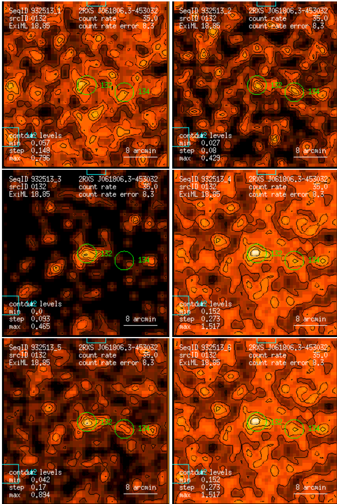
Figure 132: RASS 932513: detection 0132: band rate images, Gaussian filter: (1) PSPC channels 11 – 41, (2) 52 – 90, (3) 91 – 201, (4) 11 – 235, (5) 52 – 201, (6) 11 – 201. Broad band rates in counts/ks. Band rate contour levels in counts/ks/arcmin 2 .
