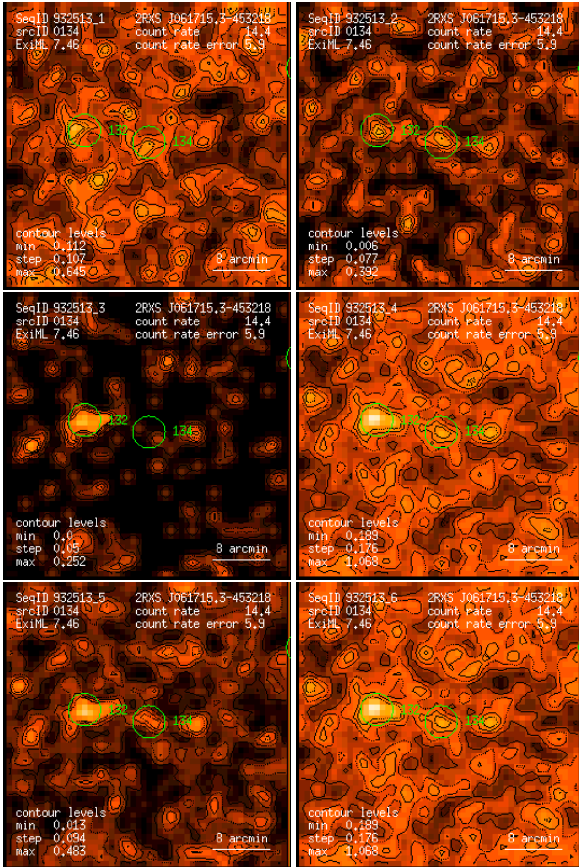
Figure 134: RASS 932513: detection 0134: band rate images, Gaussian filter: (1) PSPC channels 11 – 41, (2) 52 – 90, (3) 91 – 201, (4) 11 – 235, (5) 52 – 201, (6) 11 – 201. Broad band rates in counts/ks. Band rate contour levels in counts/ks/arcmin 2 .
