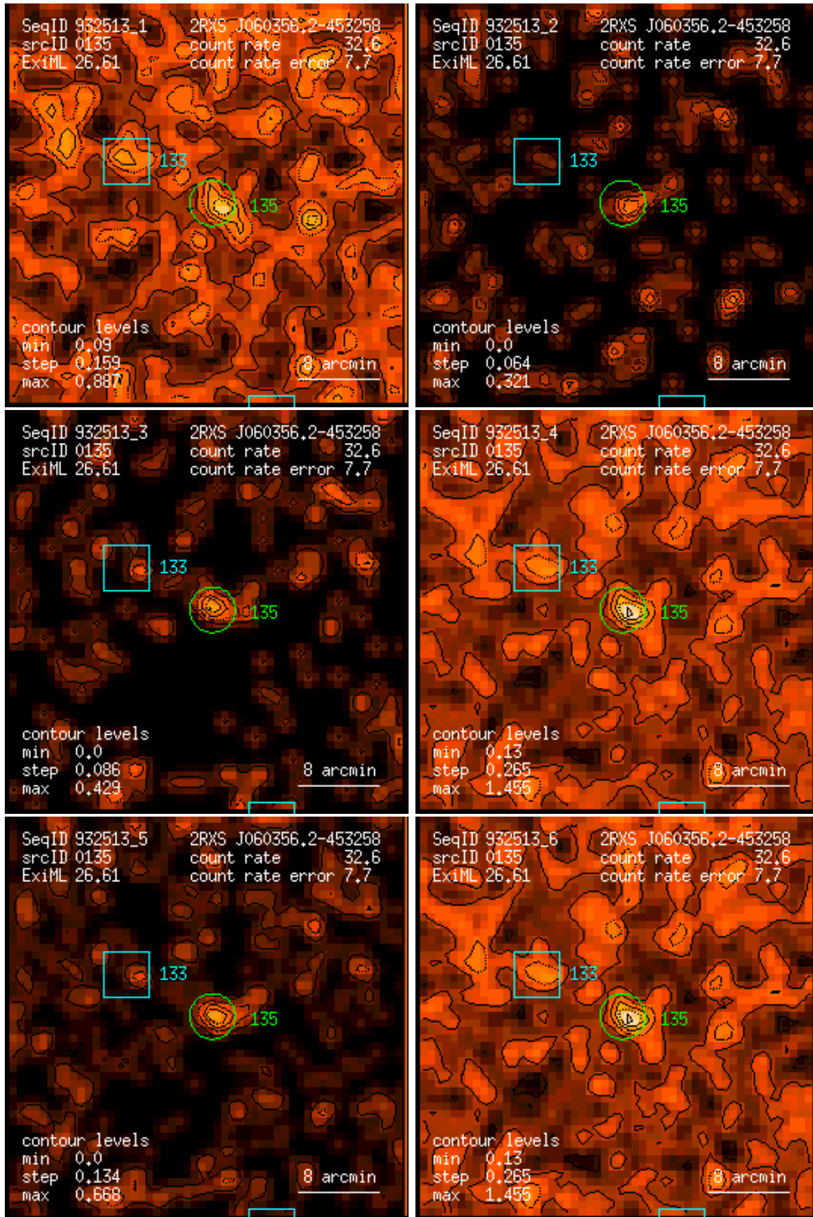
Figure 135: RASS 932513: detection 0135: band rate images, Gaussian filter: (1) PSPC channels 11 – 41, (2) 52 – 90, (3) 91 – 201, (4) 11 – 235, (5) 52 – 201, (6) 11 – 201. Broad band rates in counts/ks. Band rate contour levels in counts/ks/arcmin 2 .
