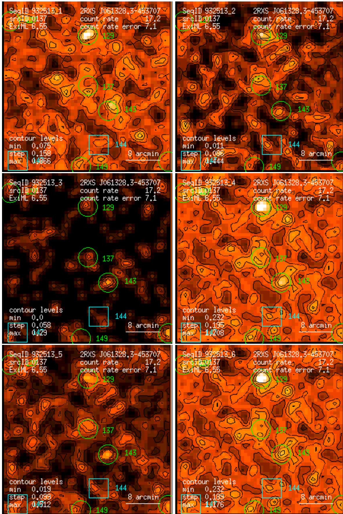
Figure 137: RASS 932513: detection 0137: band rate images, Gaussian filter: (1) PSPC channels 11 – 41, (2) 52 – 90, (3) 91 – 201, (4) 11 – 235, (5) 52 – 201, (6) 11 – 201. Broad band rates in counts/ks. Band rate contour levels in counts/ks/arcmin 2 .
