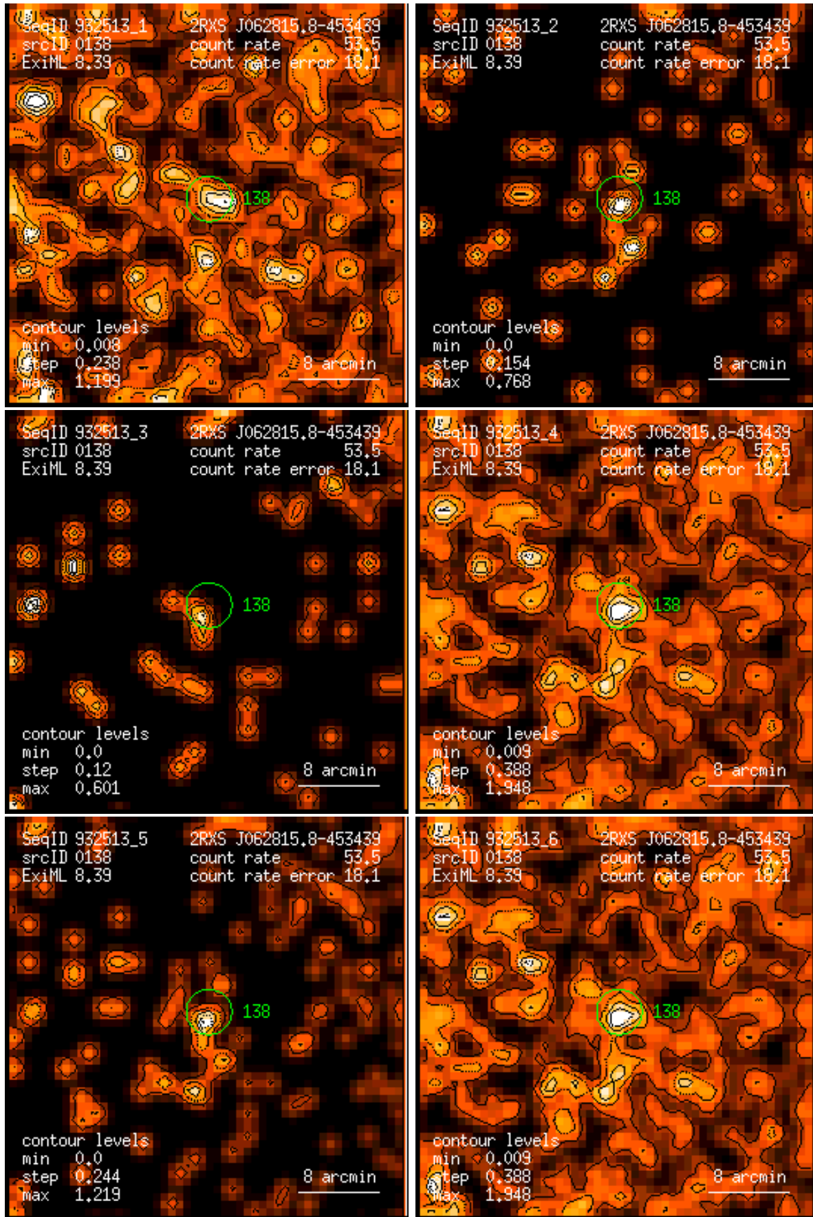
Figure 138: RASS 932513: detection 0138: band rate images, Gaussian filter: (1) PSPC channels 11 – 41, (2) 52 – 90, (3) 91 – 201, (4) 11 – 235, (5) 52 – 201, (6) 11 – 201. Broad band rates in counts/ks. Band rate contour levels in counts/ks/arcmin 2 .
