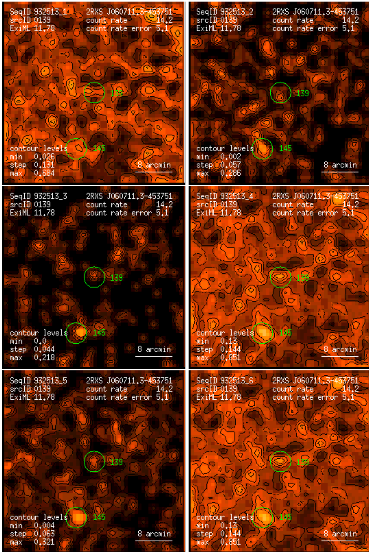
Figure 139: RASS 932513: detection 0139: band rate images, Gaussian filter: (1) PSPC channels 11 – 41, (2) 52 – 90, (3) 91 – 201, (4) 11 – 235, (5) 52 – 201, (6) 11 – 201. Broad band rates in counts/ks. Band rate contour levels in counts/ks/arcmin 2 .
