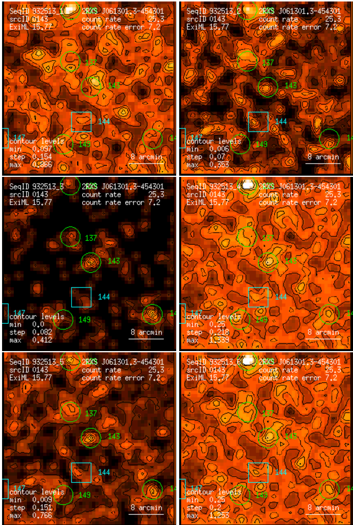
Figure 143: RASS 932513: detection 0143: band rate images, Gaussian filter: (1) PSPC channels 11 – 41, (2) 52 – 90, (3) 91 – 201, (4) 11 – 235, (5) 52 – 201, (6) 11 – 201. Broad band rates in counts/ks. Band rate contour levels in counts/ks/arcmin 2 .
