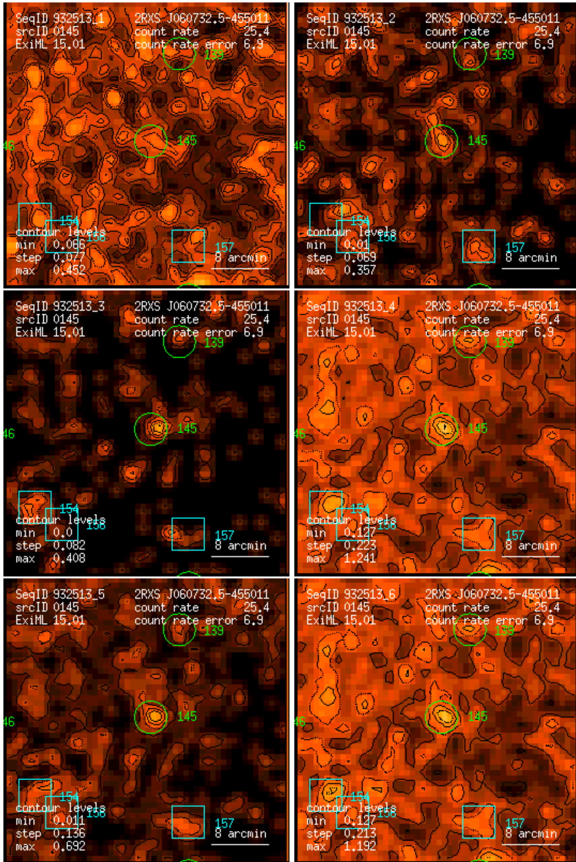
Figure 145: RASS 932513: detection 0145: band rate images, Gaussian filter: (1) PSPC channels 11 – 41, (2) 52 – 90, (3) 91 – 201, (4) 11 – 235, (5) 52 – 201, (6) 11 – 201. Broad band rates in counts/ks. Band rate contour levels in counts/ks/arcmin 2 .
