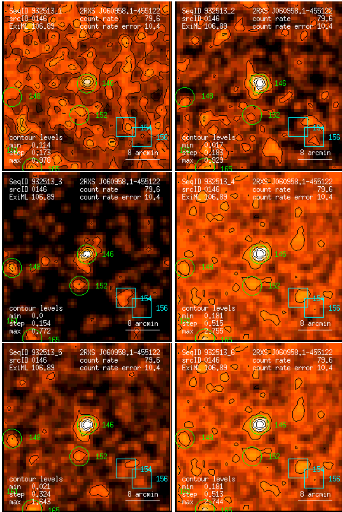
Figure 146: RASS 932513: detection 0146: band rate images, Gaussian filter: (1) PSPC channels 11 – 41, (2) 52 – 90, (3) 91 – 201, (4) 11 – 235, (5) 52 – 201, (6) 11 – 201. Broad band rates in counts/ks. Band rate contour levels in counts/ks/arcmin 2 .
