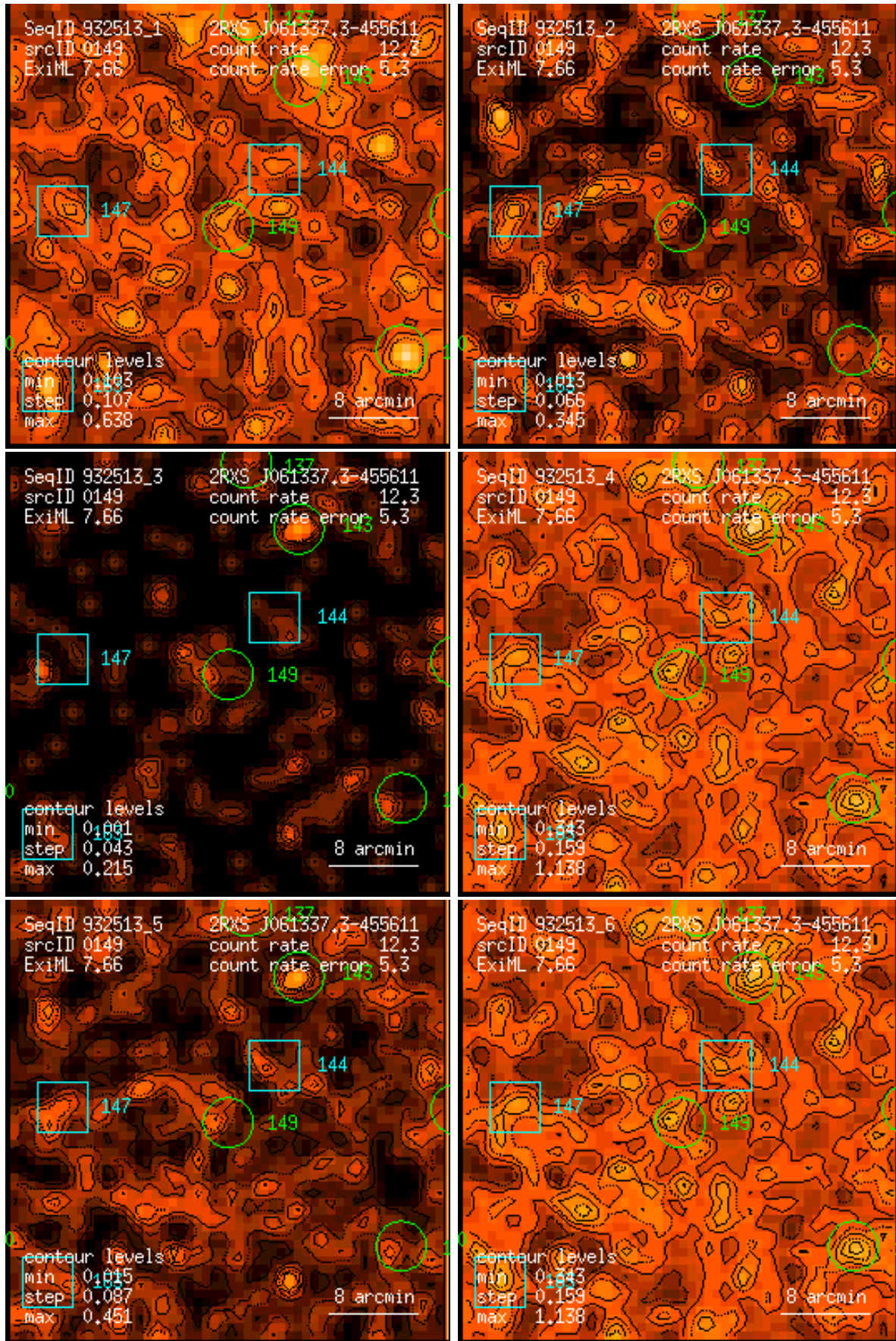
Figure 149: RASS 932513: detection 0149: band rate images, Gaussian filter: (1) PSPC channels 11 – 41, (2) 52 – 90, (3) 91 – 201, (4) 11 – 235, (5) 52 – 201, (6) 11 – 201. Broad band rates in counts/ks. Band rate contour levels in counts/ks/arcmin 2 .
